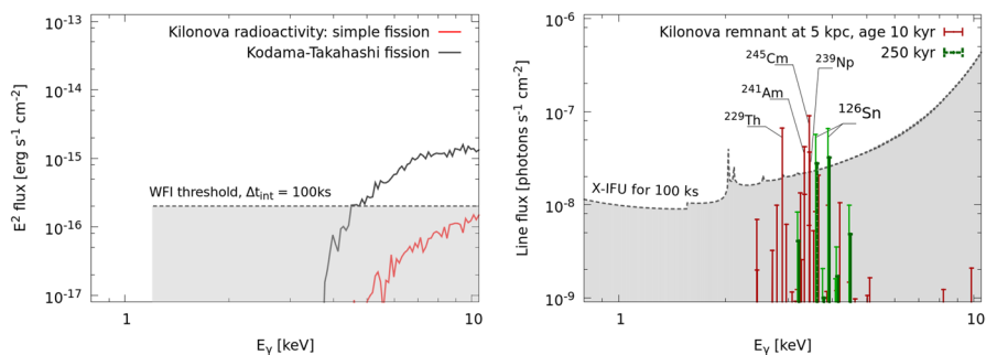
Fig. 8 Left: tentative X-ray spectra of kilonova radioactivity at a distance of 10 Mpc, integrated over 100 ks, for two representative models of nuclear fission [65]. Right: X-ray line emission from a galactic kilonova remnant at a distance of 5 kpc, for two epochs: 10 kyr (solid lines) and 250 kyr (dashed lines). X-ray spectral lines at an age < 10 kyr resulting from actinide isotopes from neutron rich r-process are shown in red. The green lines highlight X-ray emission from ^{126}\text{Sn} with the half-life of 230,000 years. The remnant is assumed to have the main r-process composition and a mass of 0.03 M_{\odot} .
