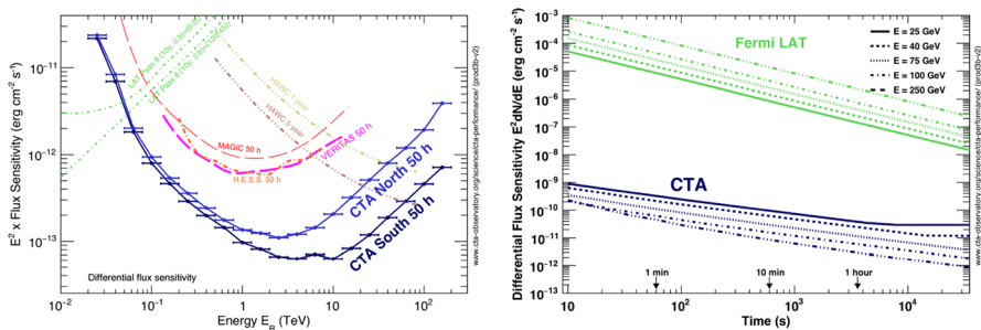
Fig. 15 Sensitivity of CTA compared to other gamma-ray observatories. Left: Comparison for persistent sources taking into account that Fermi -LAT and HAWC are wide-area detectors surveying large part of the sky, accumulating data over long periods, whereas CTA requires pointed observations. Hence the different integration times. Right: The sensitivity of CTA compared to Fermi -LAT as a function of integration time, which is relevant for transient sources like GRBs, novae, X-ray binaries, and neutron star-neutron star mergers. (Source: https://www.cta-observatory.org )
