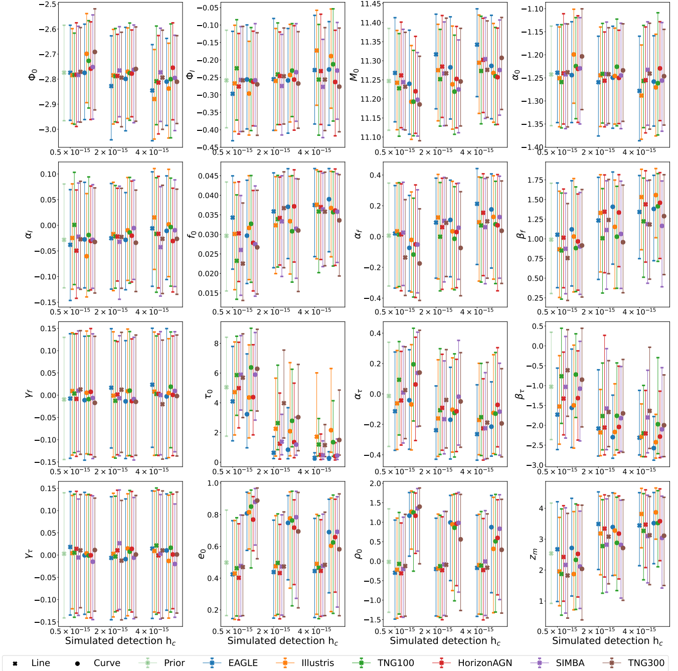
Figure 13. Median values and central 68% credible regions of the 1D marginalized posteriors from the 16 parameters using the best fit values for the BH-bulge relation for the six simulations and three different strain values and shapes. The prior distributions are indicated by the leftmost light green point in each panel. Crosses indicate straight line spectra, while circles show curved spectra. A set of six coloured points represent the results from one simulated detection case for all six simulations.
