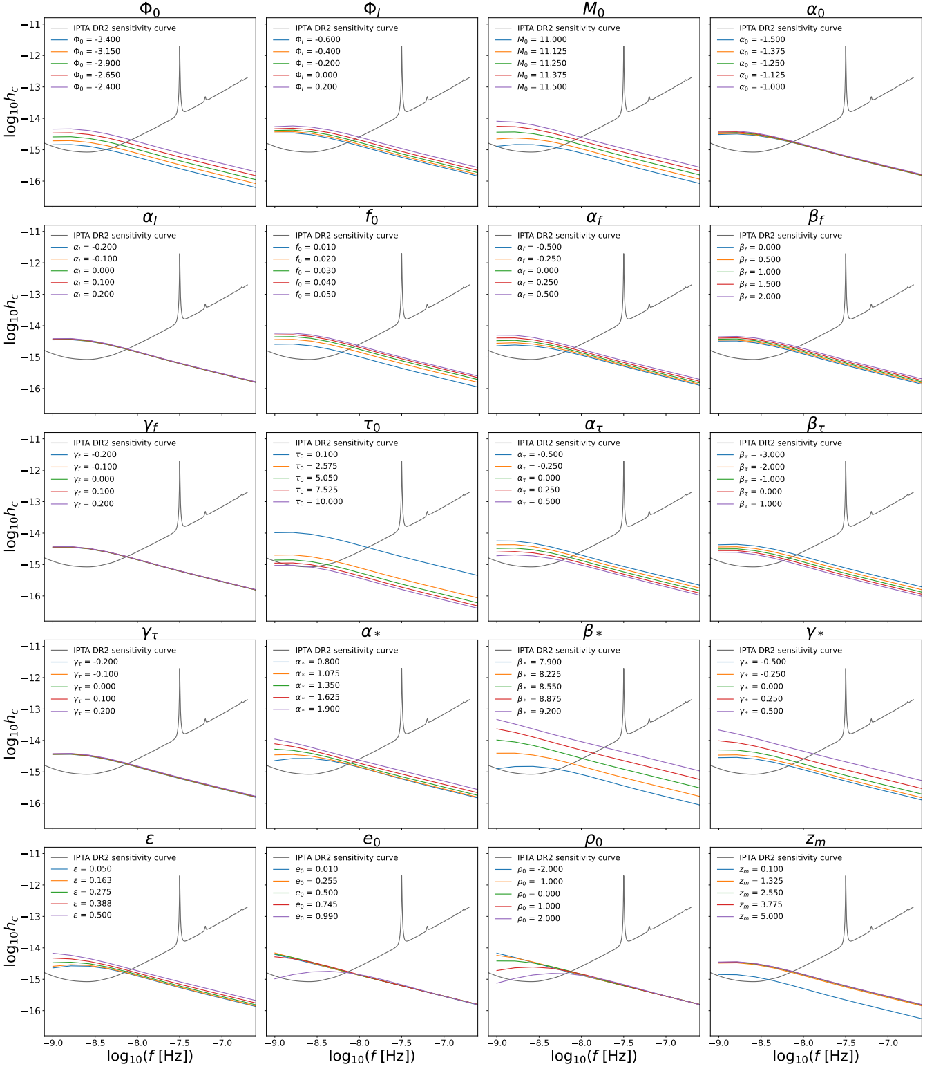
Figure A1. Effect on the GWB spectrum from variations of each of the 20 astrophysical parameters within the range given in Table 2 and Table 3. The default values for the parameters are set as: \Phi_0 = -2.6 , \Phi_I = -0.45 , M_0 = 11.25 , \alpha_0 = -1.15 , \alpha_I = -0.1 , f_0 = 0.02 , \alpha_f = 0.1 , \beta_f = 0.8 , \gamma_f = 0.1 , \tau_0 = 0.8 , \alpha_\tau = -0.1 , \beta_\tau = -2. , \gamma_\tau = -0.1 , \alpha_* = 1.1 , \beta_* = 8.2 , \gamma_* = -0.2 , \epsilon = 0.3 , e_0 = 0.9 , \log_{10} \rho_0 = 0.1 , z_m = 2.0 . Each panel shows the change in the GWB spectrum by varying only one parameter.
