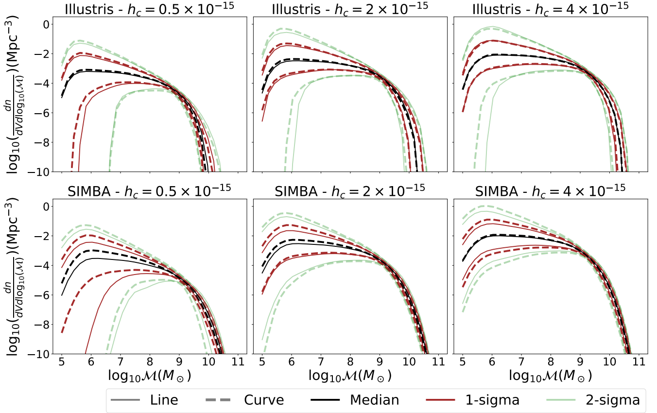
Figure 15. Same style as Figure 11, but for merger rates with respect to the chirp mass of the SMBHB using values fixed to Illustris and SIMBA in the Bayesian analysis.
