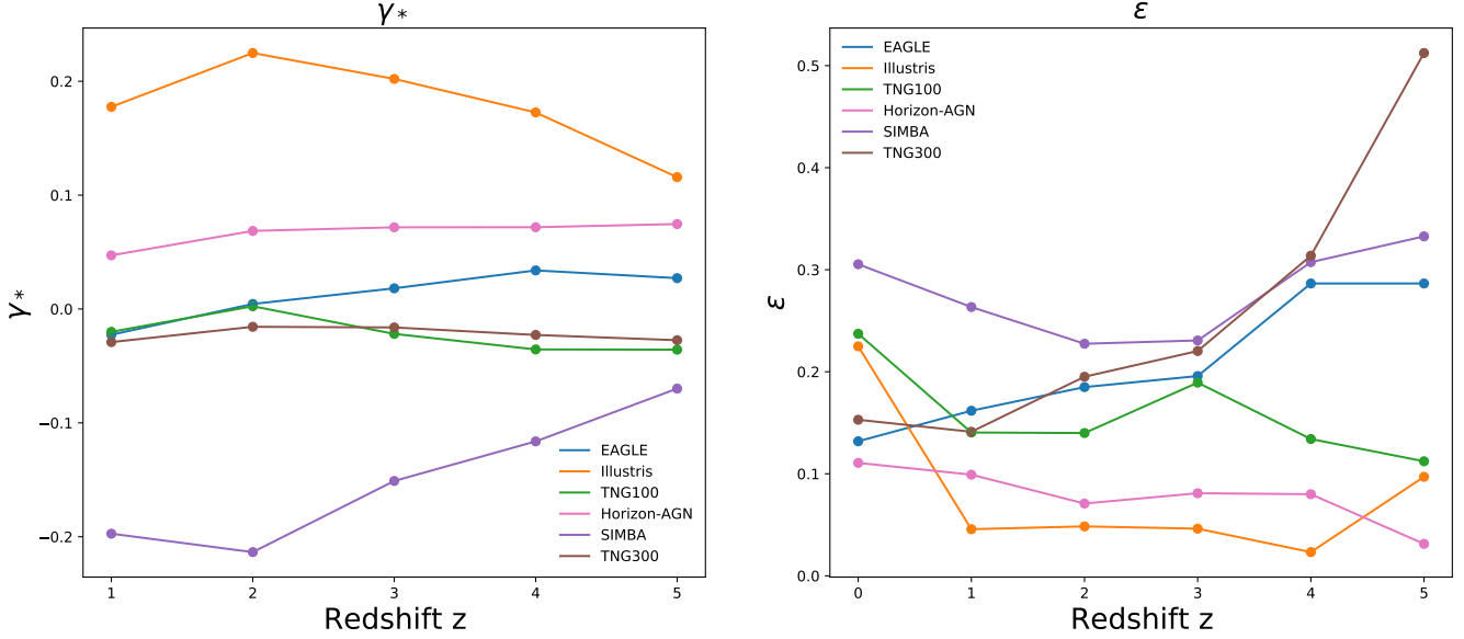
Figure 2. Variation of best fit \gamma_* and \epsilon values with redshift for the EAGLE, Illustris, TNG100, Horizon-AGN, SIMBA, and TNG300 simulations. The values are approximately constant across the redshift range for a given simulation, thus, one set of parameters ( \alpha_* , \beta_* , \gamma_* , \epsilon ) (see Table 1) can be used to represent the corresponding simulation.
