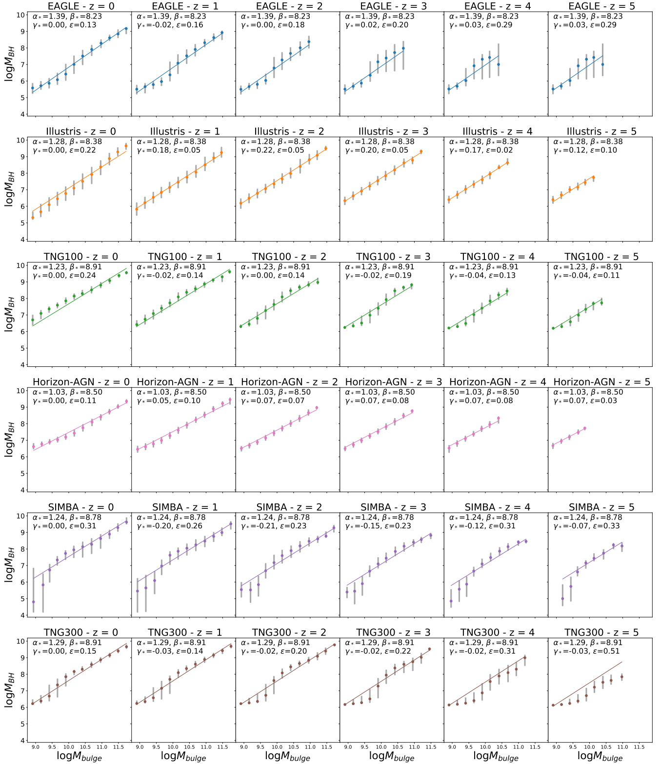
Figure 1. Best fit BH-bulge relations for the EAGLE, Illustris, TNG100, Horizon-AGN, SIMBA, and TNG300 simulations as they evolve with redshift. The BH and bulge masses with uncertainties from the simulations are consistent with the BH-bulge relations at different redshifts.
