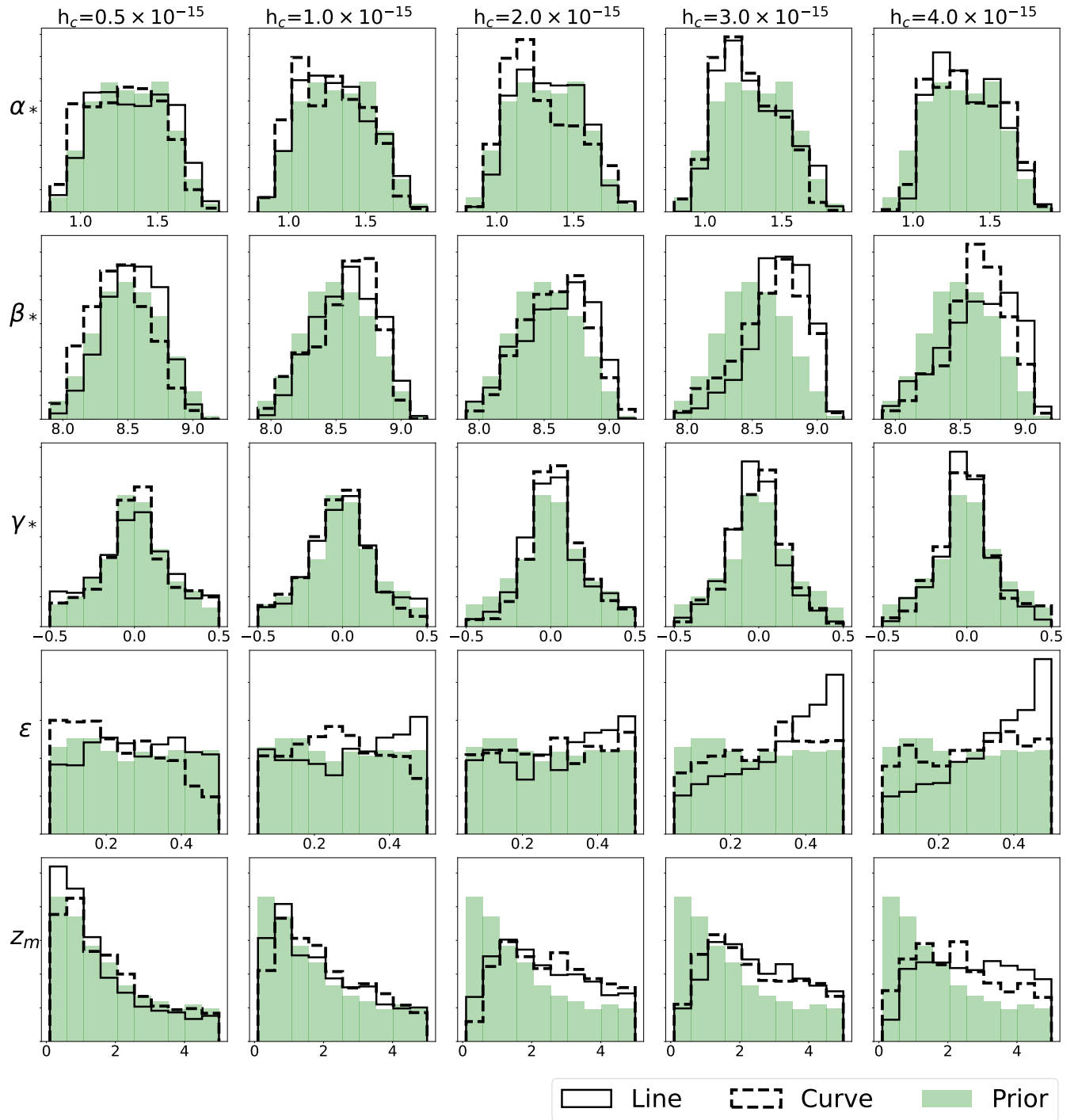
Figure 10. Posterior distributions (in black) of all the BH-bulge mass parameters including redshift variation (in the rows) as the detected characteristic strain value increases (in the columns) for both straight line (solid) and curved (dashed) spectra. For comparison the prior distributions are shown by the green shaded areas.
