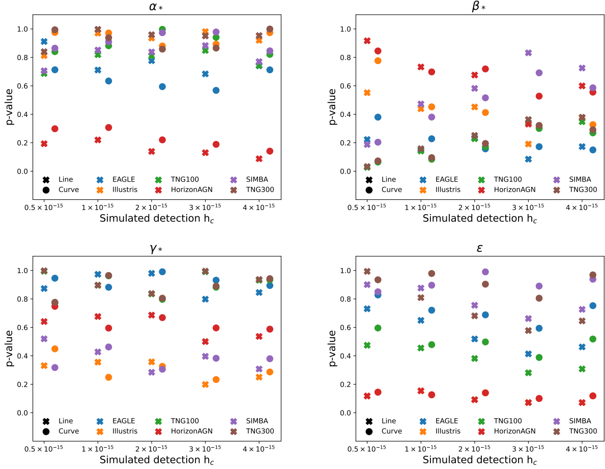
Figure 6. P-values from Kolmogorov-Smirnov tests for the fitted values from the simulations on the 1D marginalized posterior distributions for (\alpha_*, \beta_*, \gamma_*, \epsilon) . Crosses and circles indicate p-values from the straight line and curved spectra simulated detections respectively.
