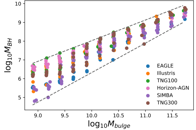
Figure 5. The BH masses of the EAGLE, Illustris, TNG100, Horizon-AGN, SIMBA, and TNG300 simulations for all redshift z \leq 5 as a function of the galaxy bulge mass. The maximum and minimum BH mass at the corresponding bulge mass are used to construct an allowed range for the BH-bulge relation, which is shown by the dashed lines.
