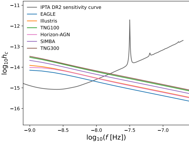
Figure 3. GWB characteristic strain spectra in the PTA range from a set of fiducial values (see Figure A1) showing the differences when using the BH-bulge mass parameters for the EAGLE, Illustris, TNG100, Horizon-AGN, SIMBA, and TNG300 simulations respectively. An analytic sensitivity curve from the IPTA DR2 (Antoniadis et al. 2022) is plotted to guide the eye.
