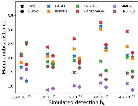
Figure 7. Mahalanobis distances between the fitted values from the simulations and the median values from the posterior constraints for all simulated data sets and both curved (circles) and straight line (crosses) spectra.
