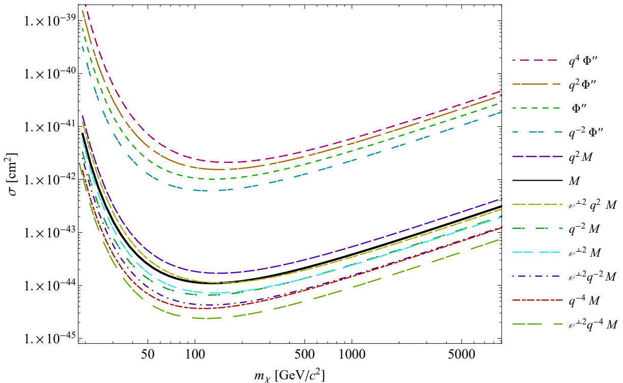
FIG. 2. DarkSide-50 90% CL exclusion curves on the cross section parameter \sigma_i for the 12 EFT terms as defined by Eq. (7). Going from top to bottom, we see a group of four curves that correspond to the nuclear response function \Phi'' times q^4 , q^2 , 1, or q^{-2} ; then a group of eight curves corresponding to the nuclear response function M times q^2 , 1, q^2 v^{\perp 2} , q^{-2} , v^{\perp 2} , q^{-2} v^{\perp 2} , q^{-4} , or q^{-4} v^{\perp 2} . The solid black curve represents the standard spin independent limits that corresponds to the current limit published in Ref. [25].
