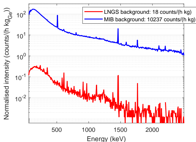
Fig. 3 Comparison between the normalised background at LNGS (lower curve, red), with a depth of 3400 mwe, and the background at the radioactivity laboratory at the University of Milano-Bicocca MIB (upper curve, blue), at sea level. Spectra are normalised in time of measurement and mass of germanium in each detector.
