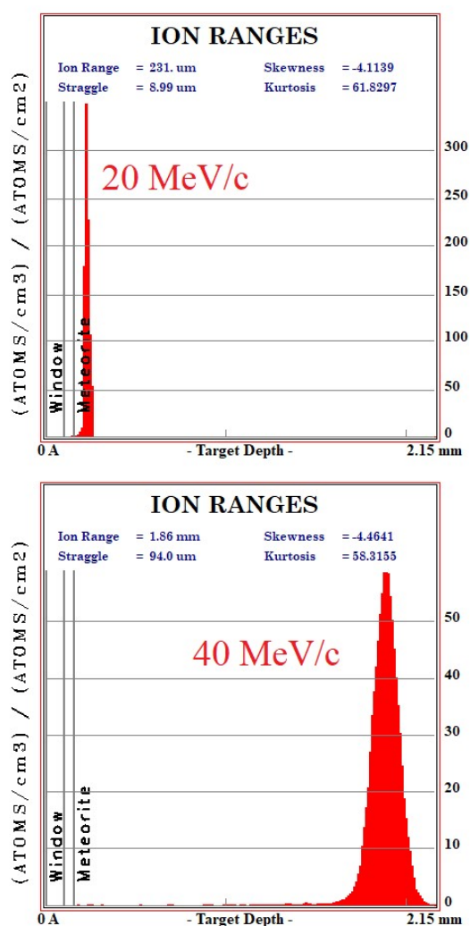
Fig. 4 Monte Carlo simulation on SRIM of the beam penetration into the sample (10k events). Upper: 20 MeV/c run, lower: 40 MeV/c run. The drawn bands show the depth of the Al layer (0.10 to 0.15 mm) and the meteorite (over 0.15 mm).
