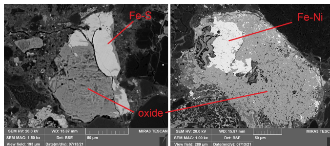
Fig. 12 Example of two iron-based relics (Fe-S left and Fe-Ni right) as seen by BSE-SEM with same level of contrast. The Fe-Ni relic appears brighter (higher atomic number Z) than Fe-S and both are surrounded by a gray area, corresponding to the oxidised metal.
