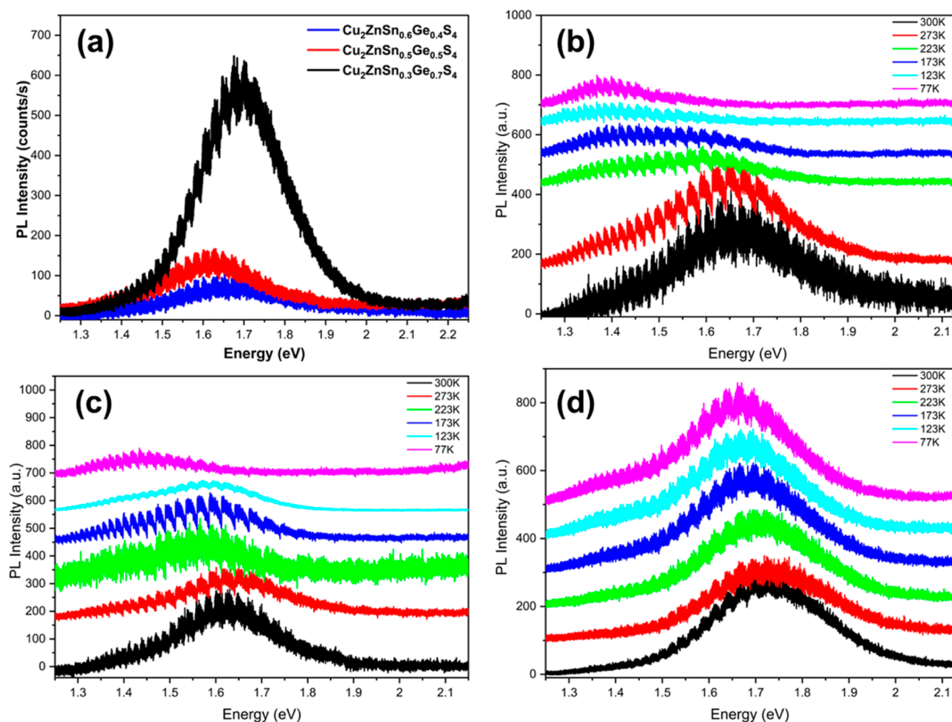
Figure 7. (a) PL measurements of \text{Cu}_2\text{ZnSn}_{0.6}\text{Ge}_{0.4}\text{S}_4 , \text{Cu}_2\text{ZnSn}_{0.5}\text{Ge}_{0.5}\text{S}_4 , and \text{Cu}_2\text{ZnSn}_{0.3}\text{Ge}_{0.7}\text{S}_4 at room temperature (excitation power of 1.2 \times 10^8 \text{ W/cm}^2 ); (b) PL measurements of the \text{Cu}_2\text{ZnSn}_{0.6}\text{Ge}_{0.4}\text{S}_4 sample at different temperatures; (c) PL measurements of the \text{Cu}_2\text{ZnSn}_{0.5}\text{Ge}_{0.5}\text{S}_4 sample at different temperatures; and (d) PL measurements of the \text{Cu}_2\text{ZnSn}_{0.3}\text{Ge}_{0.7}\text{S}_4 sample at different temperatures.
