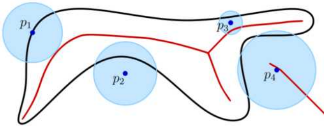
Figure 8: A planar curve (in black) and its medial axis (in red). Given some points (in dark blue), the disks centered at them (in light blue) either intersect the curve in a topological 1-disk, intersect the medial axis, or both.
