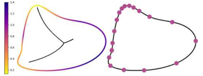
Figure 2: Left: the local feature size at each point of the curve represents its distance to the medial axis (in black). Right: a \rho -sampling of the curve with \rho = 1.0 shows that the samples are denser where the medial axis is closer to the curve.
