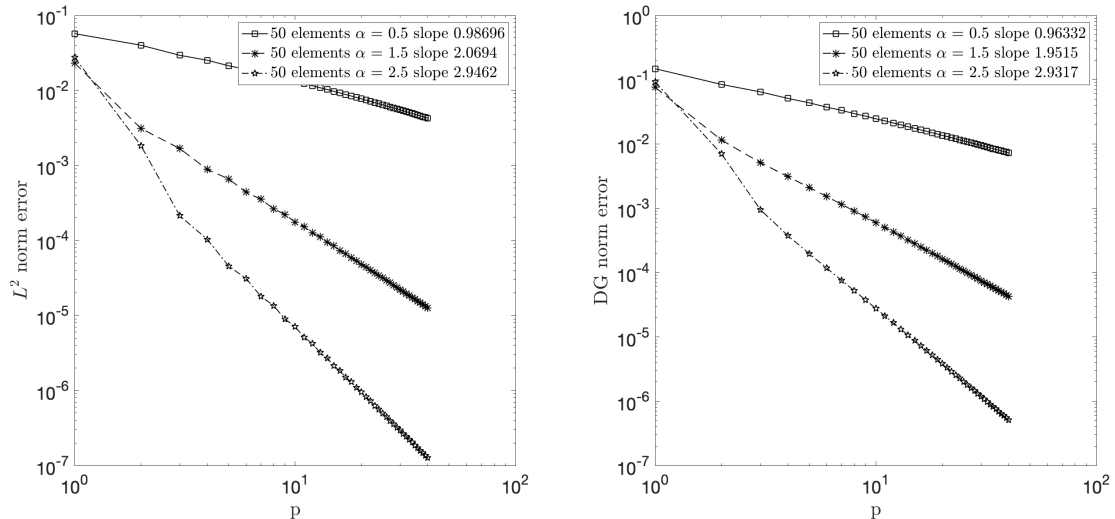
Figure 2: p -version for the case of constant convection field \beta . We consider the exact solution u in (27) and fix the triangular mesh with 50 elements as in Figure 1 so as the mesh assumptions in Section 2.1 are satisfied. The singularity lies in the interior of a cell element. Left-panel: L^2 norm error. Right-panel: DG norm error.
