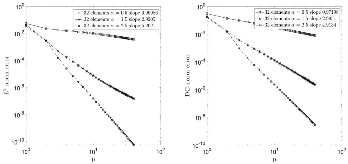
Figure 5: p -version for the case of variable convection field \beta . We consider the exact solution u in (27) and fix the triangular mesh with 32 elements as in Figure 1. The mesh assumptions in Section 2.1 are not satisfied. The singularity lies at the interface of several cell elements. Left-panel: L^2 norm error. Right-panel: DG norm error.
