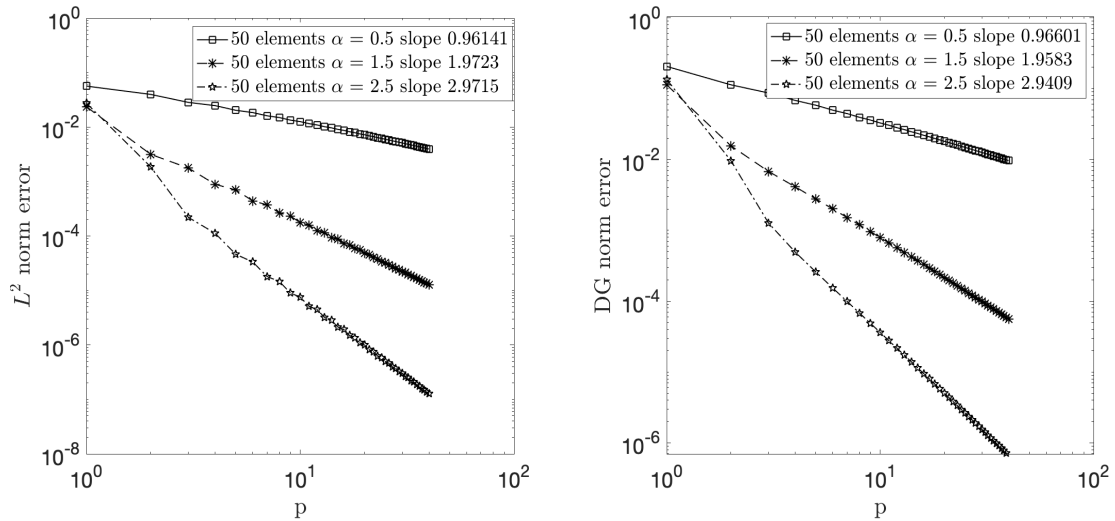
Figure 4: p -version for the case of variable convection field \beta . We consider the exact solution u in (27) and fix the triangular mesh with 50 elements as in Figure 1. The mesh assumptions in Section 2.1 are not satisfied. The singularity lies in the interior of a cell element. Left-panel: L^2 norm error. Right-panel: DG norm error.
