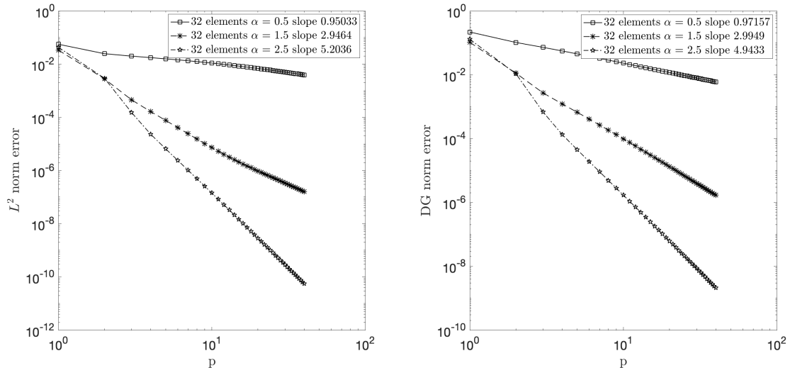
Figure 3: p -version for the case of constant convection field \beta . We consider the exact solution u in (27) and fix the triangular mesh with 32 elements as in Figure 1 so as the mesh assumptions in Section 2.1 are satisfied. The singularity lies at the interface of several cell elements. Left-panel: L^2 norm error. Right-panel: DG norm error.
