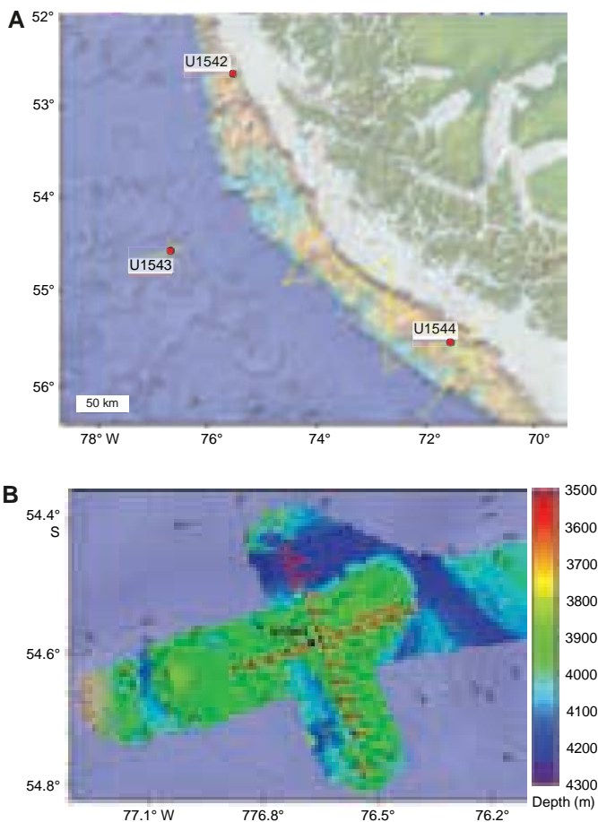
Figure F43. Oceanographic and bathymetric setting, Site U1543. A. Marine geological features. Yellow lines = seismic lines available in the region. B. Detailed bathymetry with seismic lines and shotpoints.
