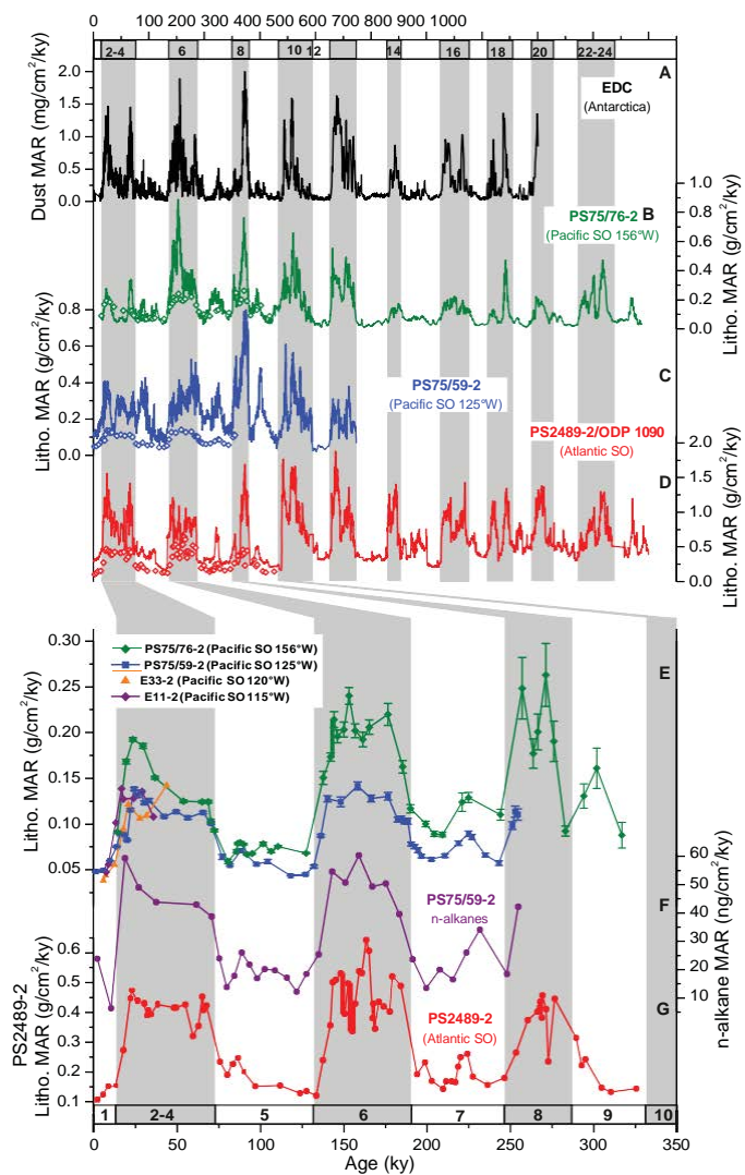
Figure F11. Changes in lithogenic mass accumulation rates (MAR Litho ) in the Pacific Southern Ocean (from Lamy et al., 2014). Open diamonds (A–C) = 230 Th-normalized MAR Litho . A. Dust MAR in the EDC ice core. B. MAR Litho Core PS75/76-2. C. MAR Litho Core PS75/59-2. D. MAR Litho ODP Leg 177 Site 1090. E. 230 Th-normalized MAR Litho Values from Cores PS75/59-2, PS75/76-2, E11-2, and E33-2. F. 230 Th-normalized C 29 and C 31 n-alkane MAR from Core PS75/59-2. G. 230 Th-normalized MAR Litho Core PS2489-2.
