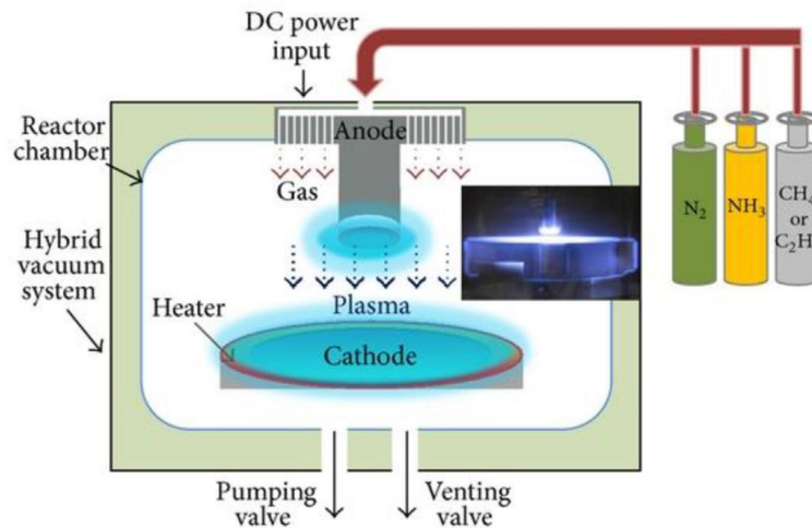
Fig. 6. Schematic representation of principles guiding the Plasma-enhanced CVD [79].
