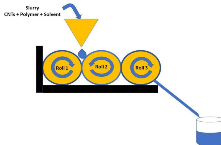
Fig. 9. Schematic of the three roll mill machine used for the calendaring process.
