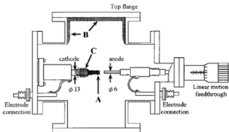
Fig. 2. Schematic representation of a typical arc-discharge apparatus [61].
