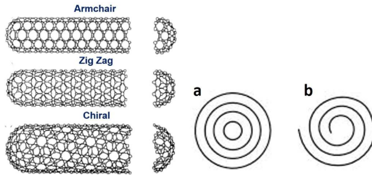
Fig. 1. On the left are shown the three models for SWCNTs structures with different chiralities. On the right, the cross-sectional view of the common Russian doll structure of concentric tubes of MWCNTs (a) and the rare parchment model (b).
