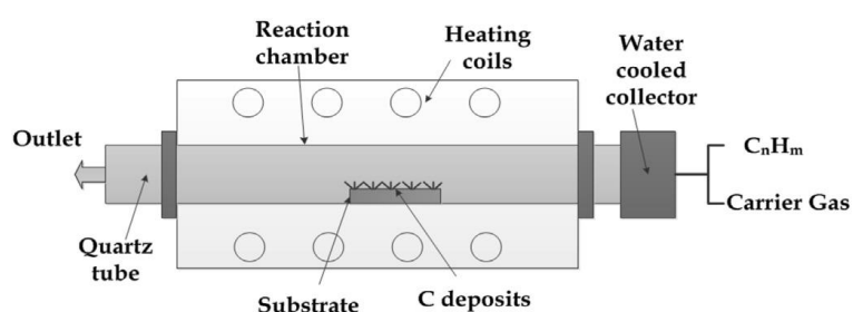
Fig. 5. Schematic representation of a CVD apparatus [65].
