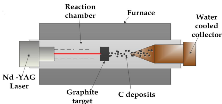
Fig. 3. Laser ablation apparatus for the production of CNTs [65].
