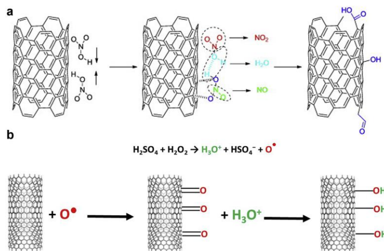
Fig. 11. a) mechanism of oxidation of nitric acid [119]; b) mechanism of oxidation of piranha solution.
