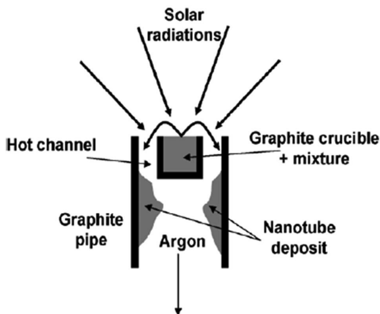
Fig. 4. Schematic representation of principles guiding the solar furnace technique [62].
