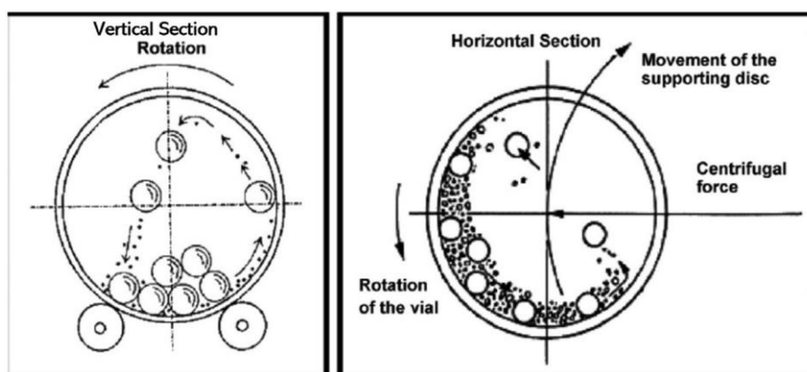
Fig. 10. Schematic representation of the balls motion during the milling process. On the left: vertical configuration (conventional ball mill). On the right: horizontal configuration (planetary ball mill) [101].
