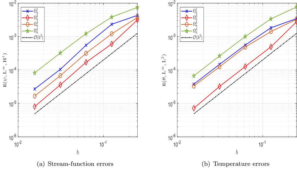
Figure 3: Accuracy assessment. Errors (6.2), using the VEM (4.1) with polynomial degrees (k, \ell) = (2, 1) , the physical parameters \nu = \kappa = 1 and the mesh families \Omega_h^i, i = 1, \dots, 4 .
