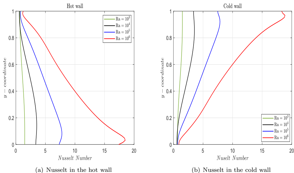
Figure 7: Natural convection cavity. Nusselt number along the hot wall (left) and the cold wall (right) for varying Rayleigh numbers, using the VEM (4.1) and mesh \Omega_h^5 , with h = 1/64 .
