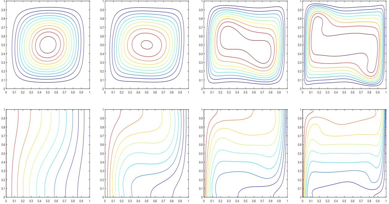
Figure 6: Natural convection cavity: streamlines (top panels) and isotherms (bottom panels), for Ra = 10^3, 10^4, 10^5 and 10^6 , respectively (from left to right).
