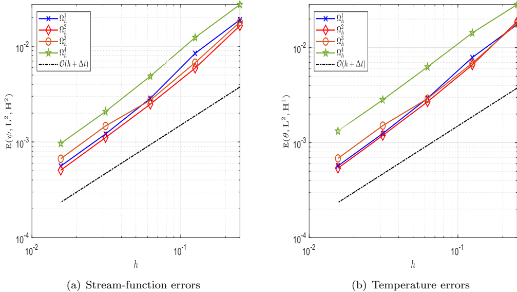
Figure 2: Accuracy assessment. Errors (6.1) for simultaneous space and time refinements, using the VEM (4.1) with polynomial degrees (k, \ell) = (2, 1) , physical parameters \nu = \kappa = 1 and the mesh families \Omega_h^i , i = 1, \dots, 4 .
