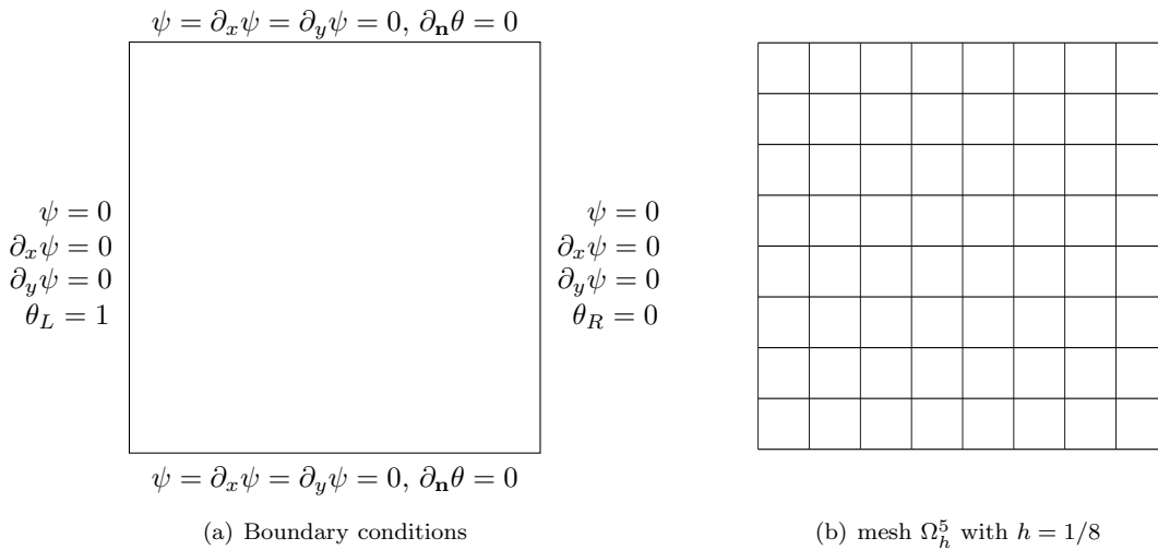
Figure 5: Natural convection cavity. Boundary conditions and domain discretized with mesh \Omega_h^5 .
