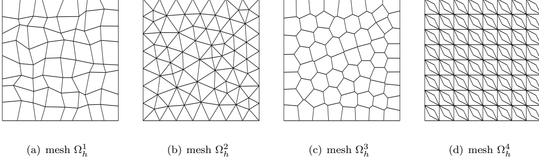
Figure 1: Domain discretized with different meshes.
