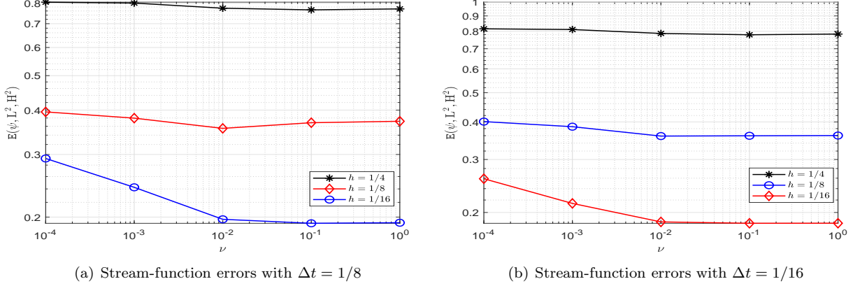
Figure 4: Small viscosity test. Errors (6.1) of the VEM (4.1), for different values of \nu and \kappa = 1 , using the meshes \Omega_h^2 , polynomial degrees (k, \ell) = (2, 1) .
