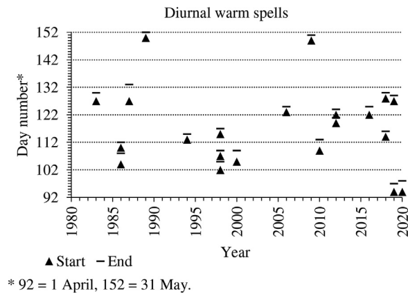
Fig. 2. Diurnal warm spell duration index (43.9 °C for 3 or more consecutive days) in Niamey, April–May 1980–2020.
