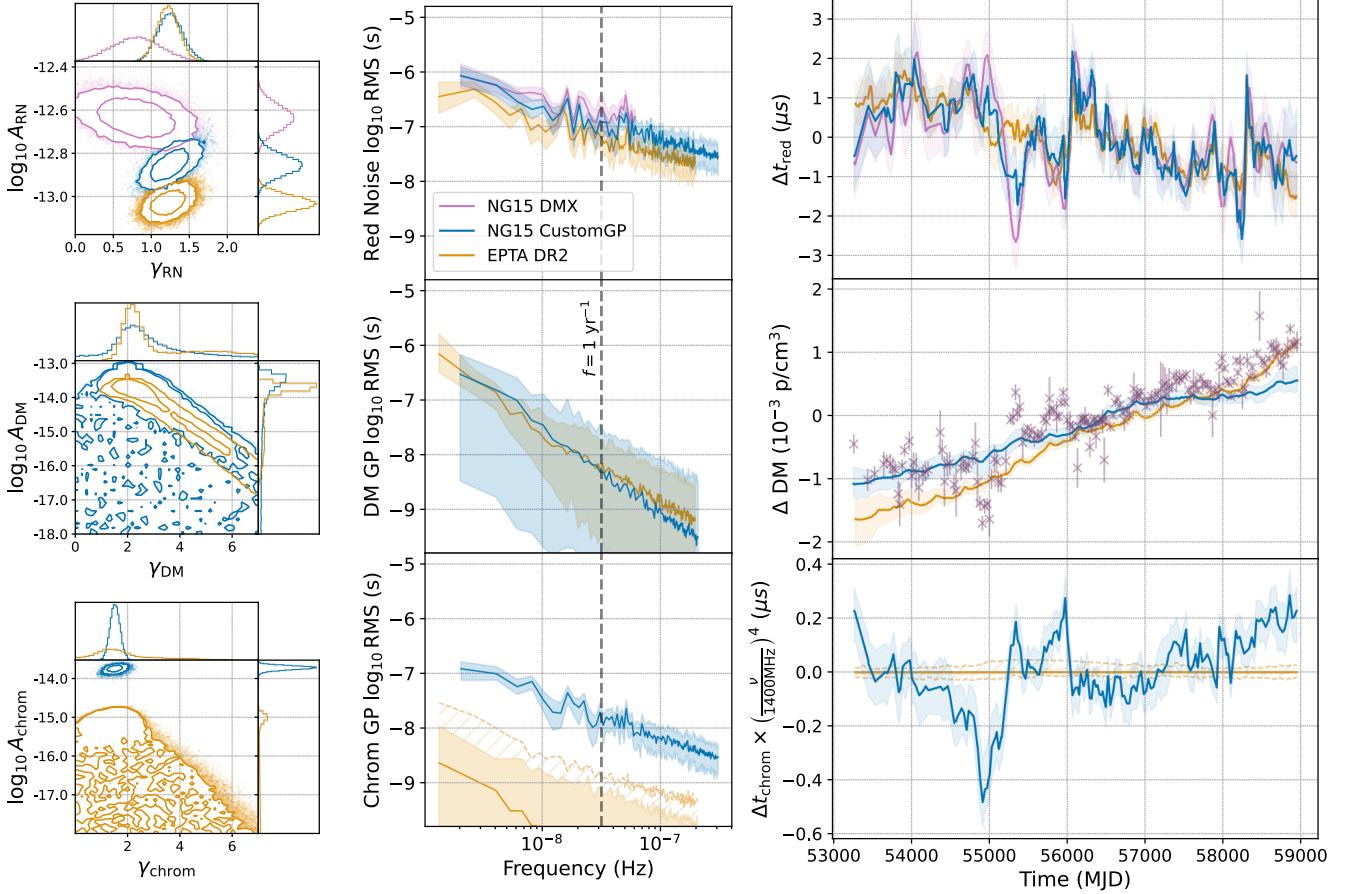
Figure 4. PSR J1012+5307 – Each noise model fails to mitigate anti-correlations between chromatic noise and a shallow-spectrum achromatic red noise process in NG15 . J1012+5307 features a peculiar shallow-spectrum ARN process, modeled in CustomGP using N_{\text{freqs}} = 150 , following Chalumeau et al. (2022) . Using CustomGP , NG15 and EPTA DR2 have the same ARN spectral index and share many common features in the time domain, including sharp spikes near MJDs 56100 and 58350. However, the NG15 ARN spectrum features excess power near 50 nHz, which is not seen in EPTA DR2 . ARN variations near MJD 55000 and MJD 56000 are anti-correlated with chromatic variations using NG15 , and the scattering-like chromatic noise detection made by NG15 is also well above the upper limit set by EPTA DR2 . See the Figure 3 caption for panel descriptions.
