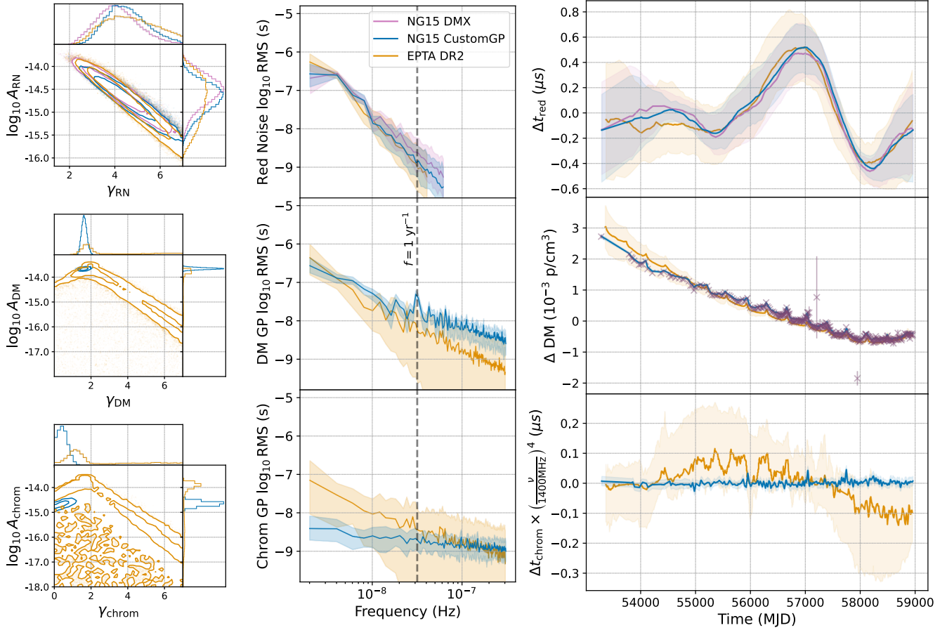
Figure 9. PSR J1909–3744 – Achromatic red noise is robust to the choice of chromatic noise model. PSR J1909–3744’s ARN in NG15 experiences little to no change going from DMX to CustomGP , indicating any errors in chromatic noise mitigation are small and decoupled from ARN. ARN characterization is also remarkably consistent between NG15 and EPTA DR2 . Spikes in the NG15 time series for scattering-like chromatic noise are also observed near annual DM cusps, indicating they likely originate from the heliosphere. See the Figure 3 caption for panel descriptions.
