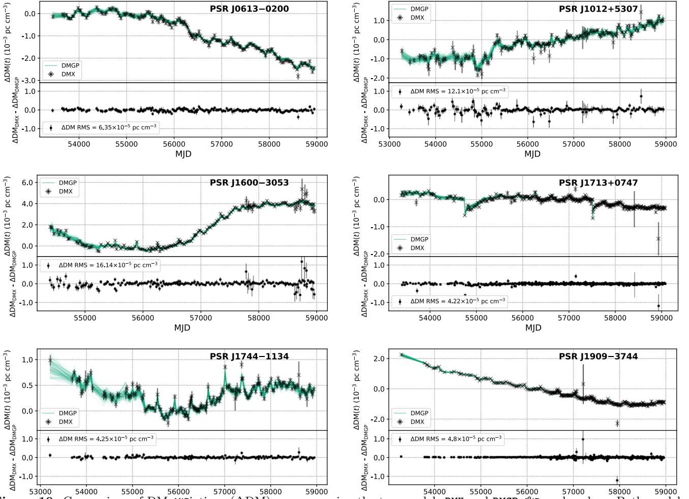
Figure 10. Comparison of DM variations ( \Delta M ) recovery using the two models DMX and DMGP, for each pulsar. Both models recover qualitatively similar trends in DM for all pulsars, however the difference in estimated DM values is largest for PSRs J1012+5307 and J1600–3053. Top panels: Time series of DMX parameters (black) superimposed with 100 DM GP realizations (turquoise). Bottom panels: Difference in estimated DM over time and root-mean-squared difference between \Delta DM values.
