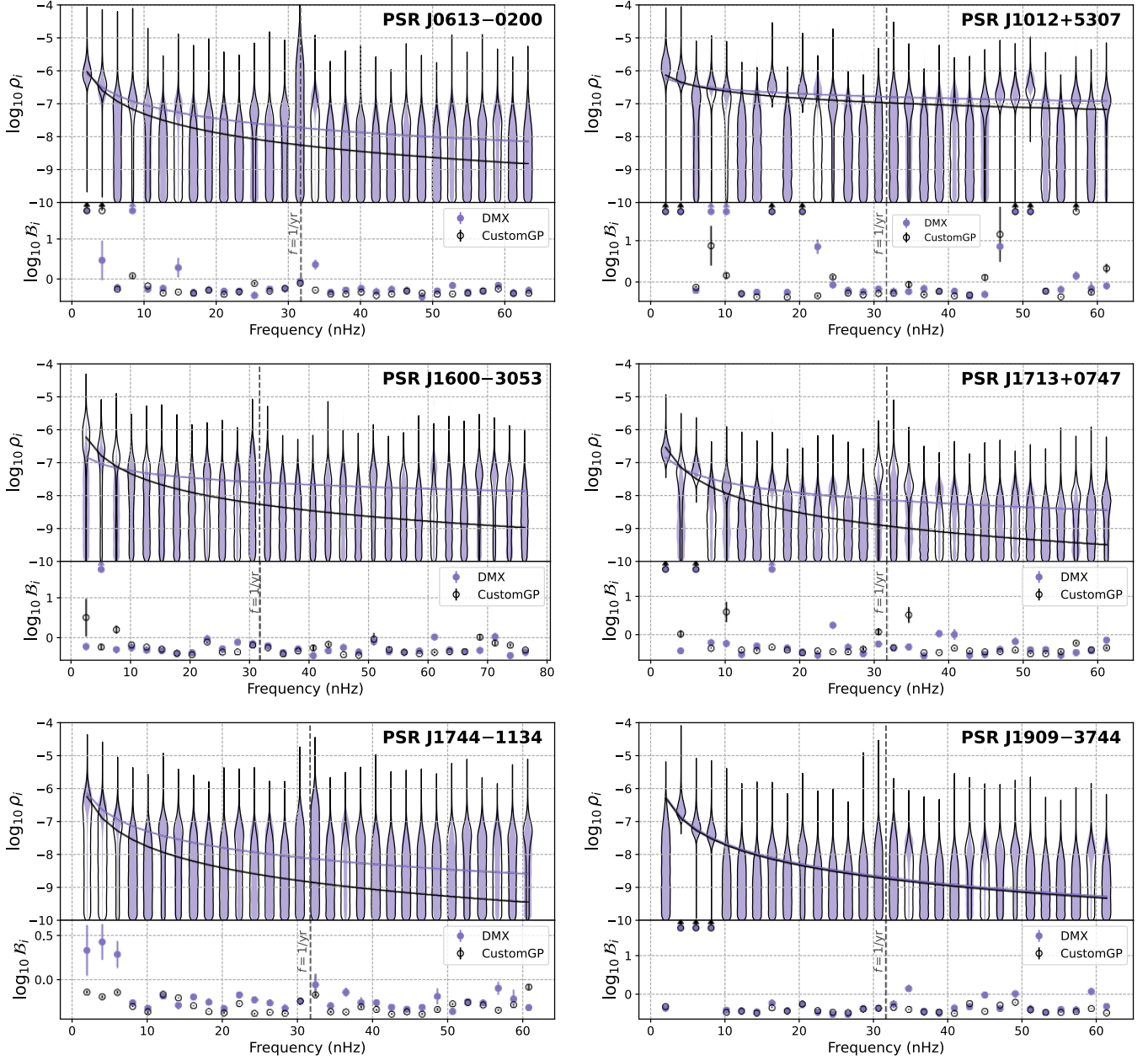
Figure 11. Power spectra and Bayes Factors using a free-spectral PSD for each pulsar, under the two models: DMX and CustomGP. Top panels show the posteriors for the log-scaled residual power \log_{10} \rho_i at each frequency, in units of excess timing delay. Bottom panels show log-scaled Bayes factors \log_{10} \mathcal{B}_i indicating the statistical significance of excess power in each frequency bin. For each pulsar, changes to \rho_i are isolated to a few key frequencies, but still influence the inferred power law noise parameters (Figure 2).
