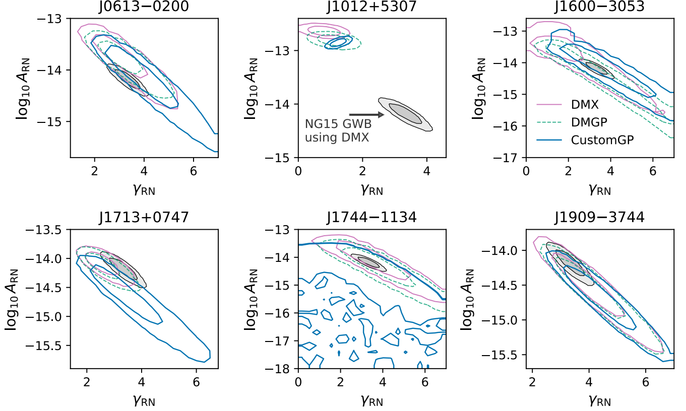
Figure 2. Accounting for non-dispersive chromatic noise using the CustomGP model noticeably affects achromatic red noise posteriors for multiple pulsars within NG15. Posterior distributions for the six pulsars’ ARN parameters using the DMX (solid purple), DMGP (dashed green), and CustomGP (solid blue) models. Since the GWB makes up a portion of all pulsars ARN budget, the GWB parameters inferred from NG15.GWB using the DMX model for all pulsars is included in gray. The inferred ARN posteriors change the most substantially for PSRs J1713+0747 and J1012+5307 using CustomGP. PSRs J0613–0200, J1600–3053, and J1744–1134 also feature noticeable changes to their ARN parameters at a less significant level. PSR J1909–3744’s ARN parameters are the least affected the choice of noise model. The apparent shift of PSR J1713+0747’s ARN parameters away from the inferred GWB parameters indicates its choice of noise model is likely to affect GWB spectral characterization.
