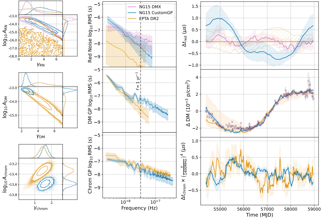
Figure 5. PSR J1600–3053 – Achromatic red noise is highly sensitive to the chromatic noise parameters, which are inconsistent between NG15 and EPTA DR2. CustomGP mitigates short-timescale chromatic noise, resulting in a steeper ARN spectrum than DMX. NG15 and EPTA DR2 both agree on the presence of strong DM and scattering-like variations, but the scattering-like chromatic noise amplitude and DM noise spectral index are both lower using NG15. In the time-domain, several chromatic features are present in both data sets, but neither data set agrees on whether the DM or scattering-like chromatic term should mitigate them. See the Figure 3 caption for panel descriptions.
