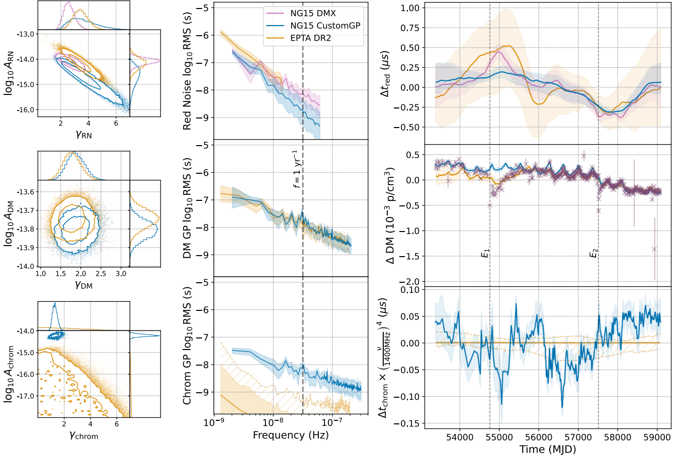
Figure 6. PSR J1713+0737 – Simultaneous achromatic red noise and DM variations near the second transient timing event are decoupled using CustomGP. The times of events E_1 and E_2 are indicated by the dashed lines. Using DMX, E_2 manifests as a dip in both the NG15 DMX time series and time-domain ARN realizations. Modeling E_2 in CustomGP using a free chromatic index successfully decouples this event from both the ARN and DM noise. This lowers the value of \log_{10} A_{\text{RN}} and widens the posterior on \gamma_{\text{RN}} . However, the ARN and scattering-like chromatic noise parameters in NG15 are in tension with EPTA DR2. See the Figure 3 caption for panel descriptions.
