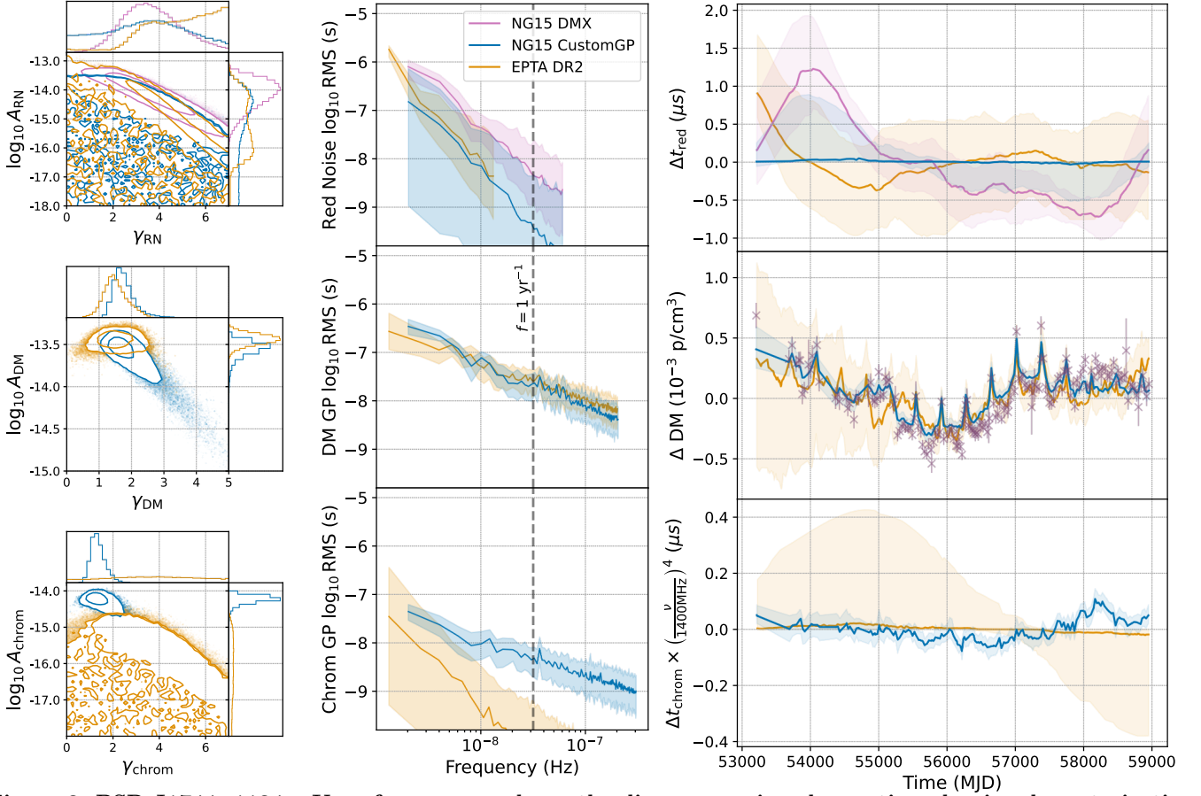
Figure 8. PSR J1744–1134 – Use of CustomGP reduces the discrepancy in achromatic red noise characterization between NG15 and EPTA DR2. When applying CustomGP to NG15, the detection of ARN is reduced to an upper limit. This improves the consistency in ARN characterization between data sets, as indicated by their ARN spectra. However, the detection of scattering-like chromatic noise in NG15 is above the upper limit set by EPTA DR2. See the Figure 3 caption for panel descriptions.
