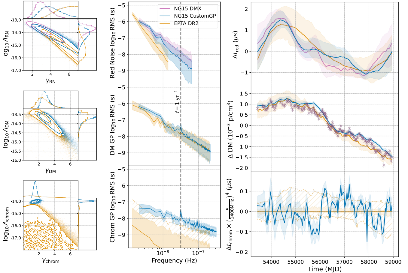
Figure 3. PSR J0613–0200 – A variation in the achromatic red noise, uniquely observed using NG15, is mitigated using CustomGP. Noise properties are displayed by column: posterior parameter distributions (left), spectra (middle), and time-domain GP realizations (right). Noise types are displayed by row: ARN (top), DM variations (middle), and scattering-like chromatic noise with \chi = 4 (bottom). Data/model in use are displayed by color: NG15 using DMX (purple), NG15 using CustomGP (blue), and EPTA DR2 (yellow). All chromatic noise spectra are referenced to a delay at 1400 MHz. A variation present in the time-domain ARN realizations near MJD 56000 using DMX is now absorbed by the chromatic noise model using CustomGP. This ARN variation is not present in EPTA DR2. The ARN spectrum is steeper and more consistent with EPTA DR2 when applying CustomGP. An annual trend in the time series of DMX parameters is now absorbed by the scattering-like chromatic model using CustomGP. However, the scattering-like chromatic noise amplitude from NG15 is above the upper limit set by EPTA DR2.
