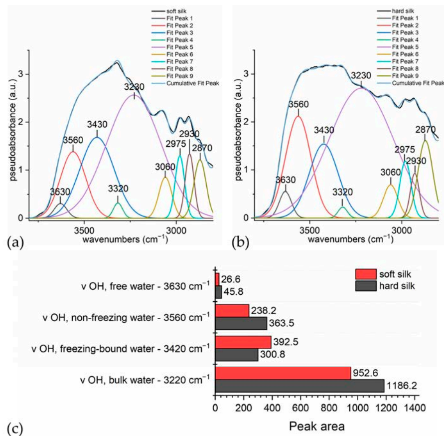
Figure 6. Deconvolution of the O-H stretching band (region 3715–2800 \text{cm}^{-1} ): (a) soft silk; (b) hard silk; (c) comparison of the peak areas for each contribution in soft and hard silk.
