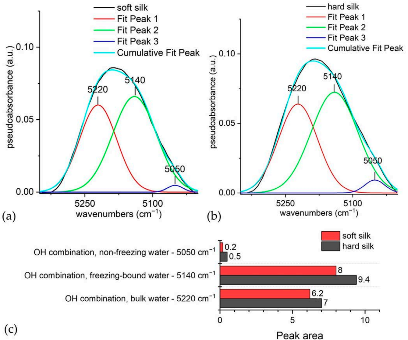
Figure 8. Deconvolution of the band at 5170 cm -1 . Deconvolution of the O-H combination band (region 5350–5000 cm -1 ): (a) soft silk; (b) hard silk; (c) comparison of the peak areas for each contribution in soft and hard silk.
