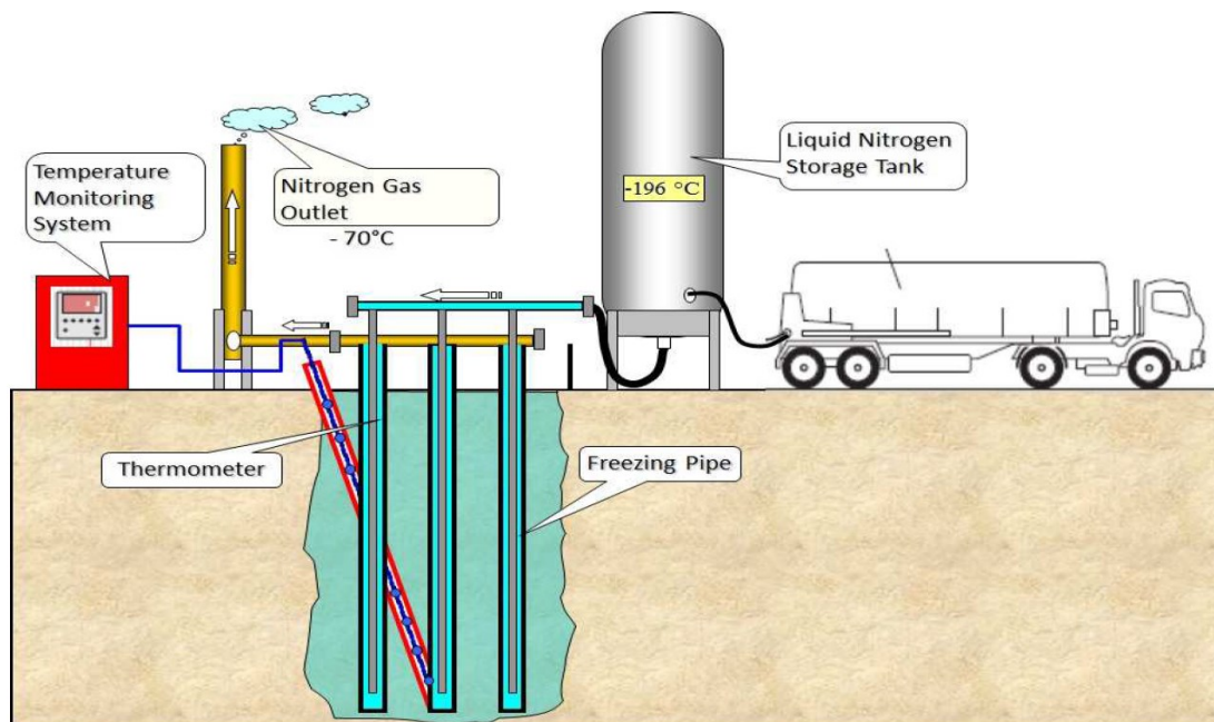
Fig. 7-8, Artificial ground freezing with nitrogen technique: direct system circuit scheme. (Mira Cattò et al. 2016)
