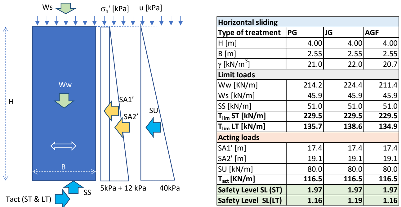
Fig. 6-5, Horizontal sliding verification of the adopted case study (ST Short Term; LT long Term).
