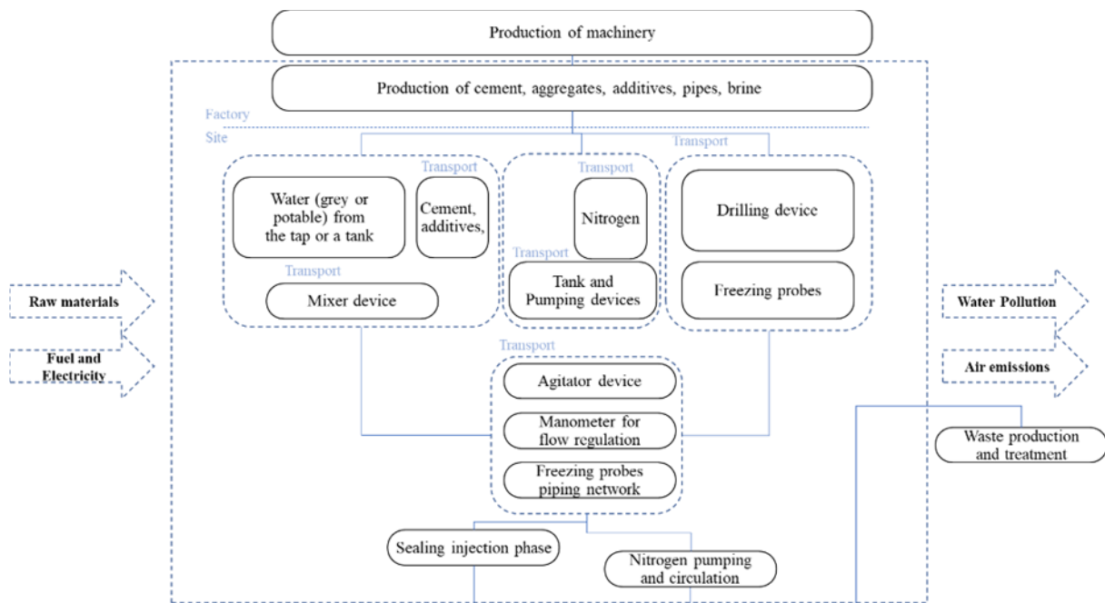
Fig. 9-10, Artificial ground freezing with nitrogen technique: LCA Process scheme.
