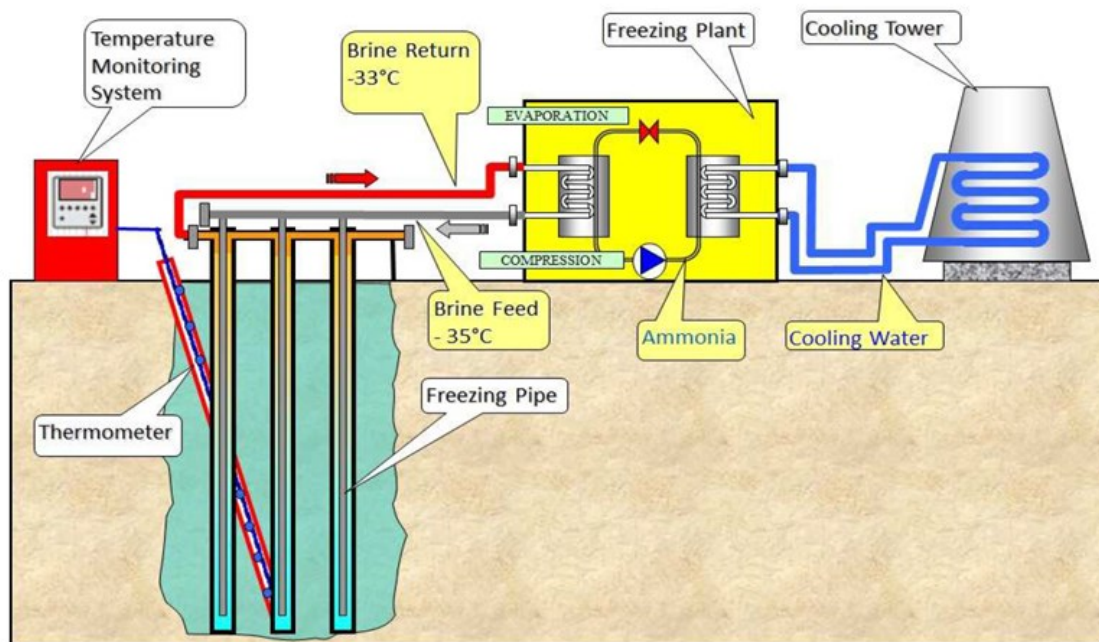
Fig. 7-6, Artificial ground freezing with brine technique: Indirect system circuit scheme (with brine). (Mira Cattò et al. 2016)
