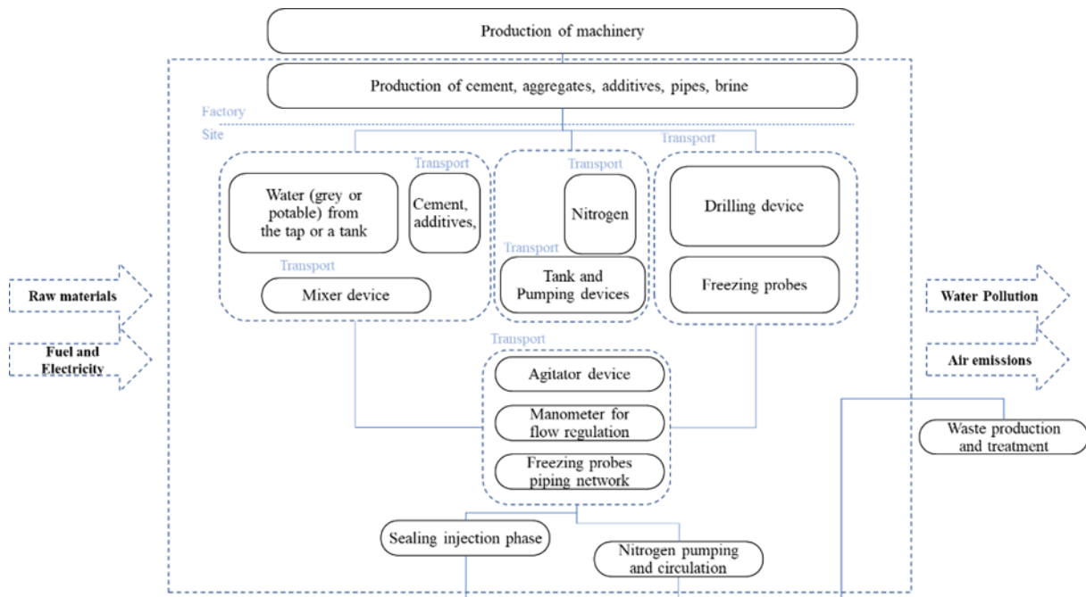
Fig. 18-24, Artificial ground freezing with nitrogen technique: LCA Process scheme.
