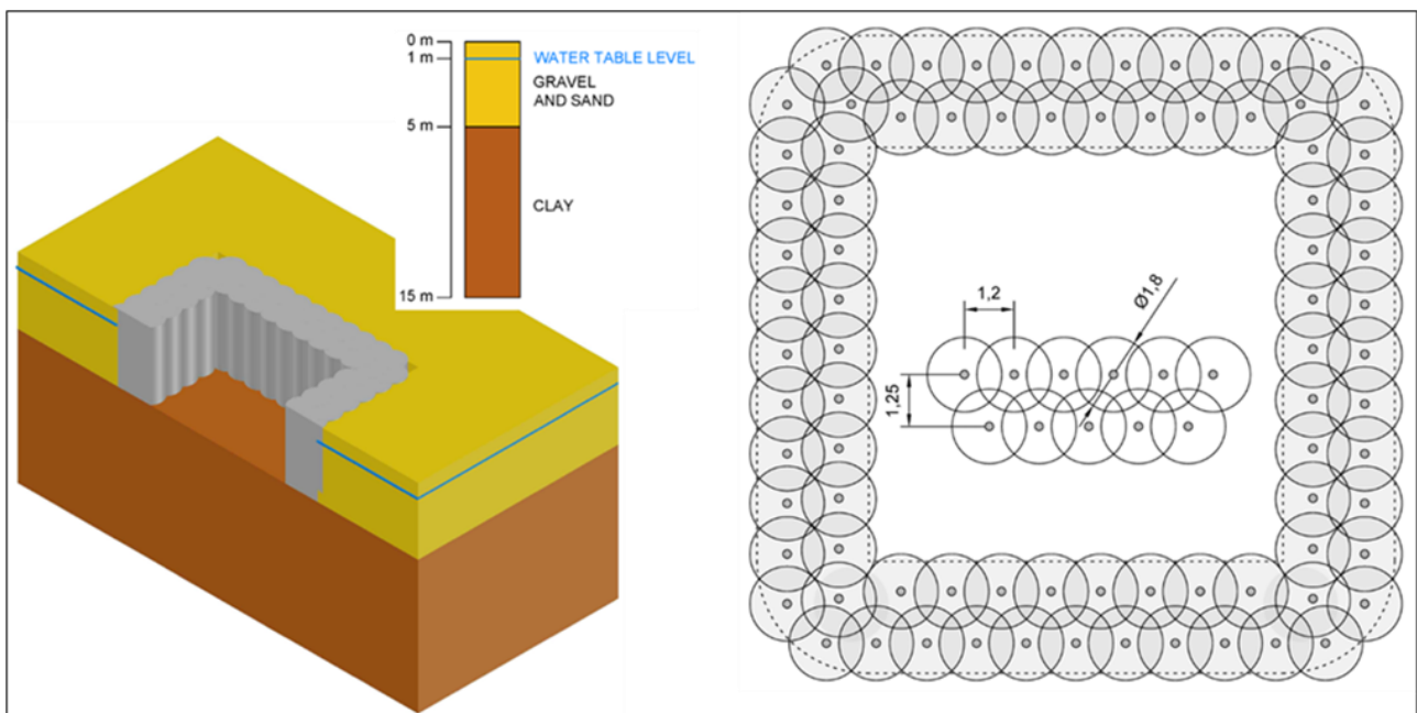
Fig. 9-7, Jet grouting with double fluid technique: geometrical data.
