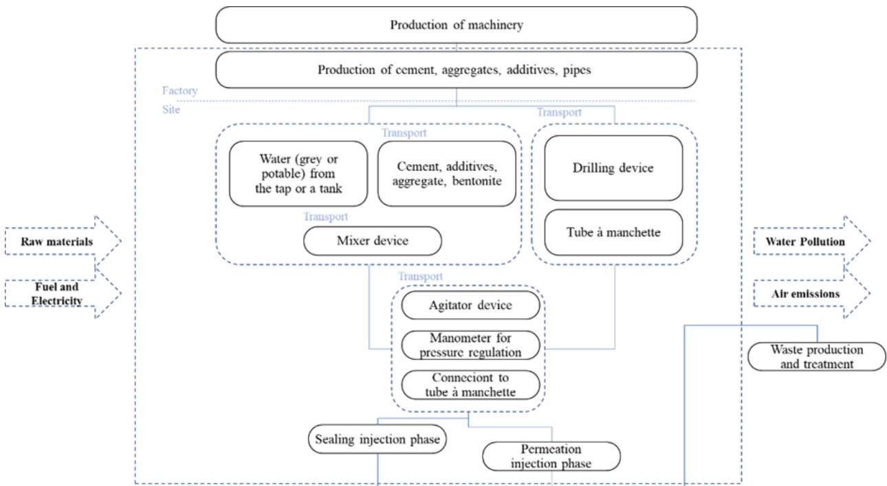
Fig. 18-1, Process scheme for LCA Analysis of the permeation grouting technique.
