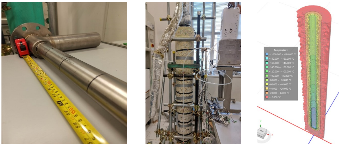
Fig. 14-5, GFLab - Ongoing laboratory test on freezing pipe (Bavaresco, 2023)
