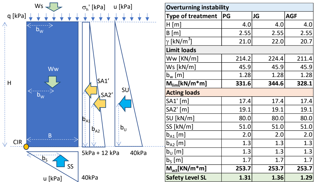
Fig. 6-4, Overturning verification of the adopted case study.
