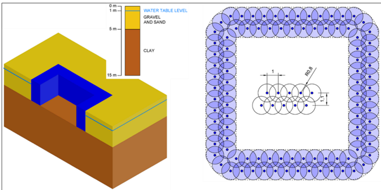
Fig. 9-8, Artificial ground freezing technique (AGF-BR and AGF-LN): geometrical data.
