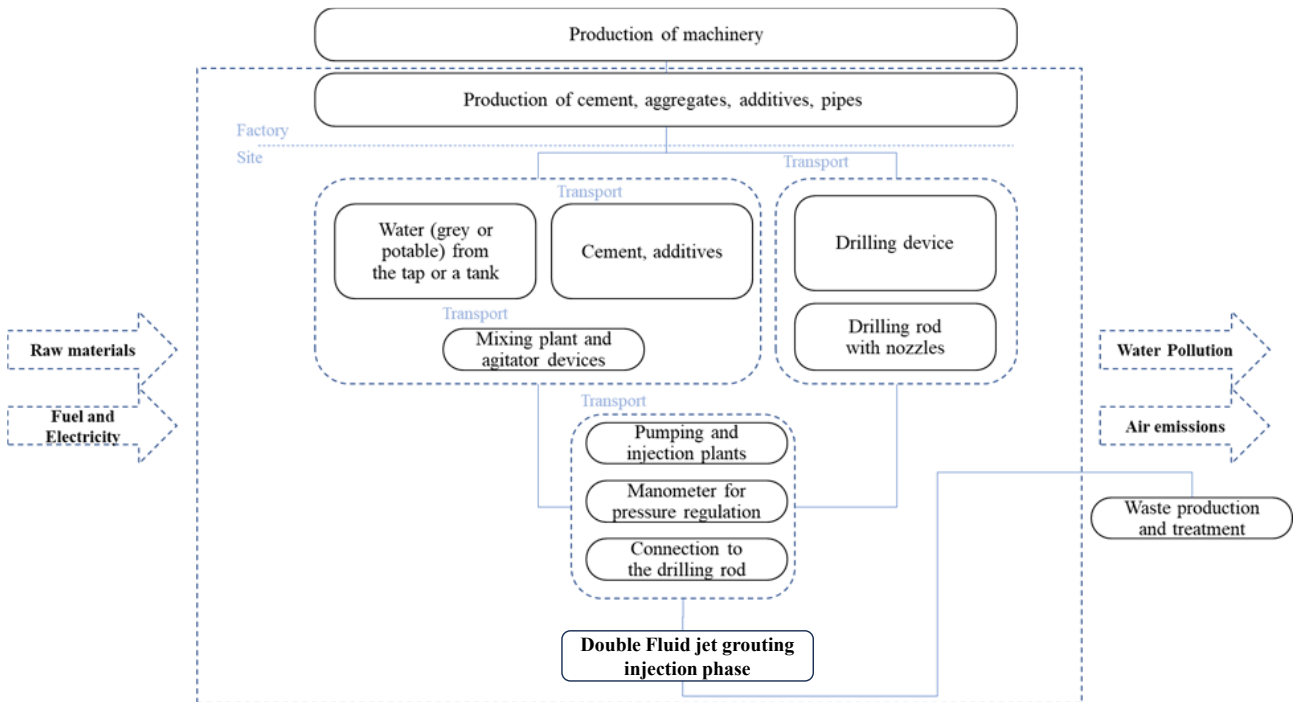
Fig. 18-13, Process scheme for LCA Analysis of the single fluid Jet Grouting technique.
