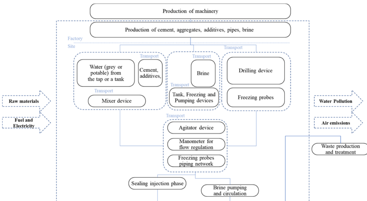
Fig. 9-9, Artificial ground freezing with brine technique: Process scheme for LCA Analysis.
