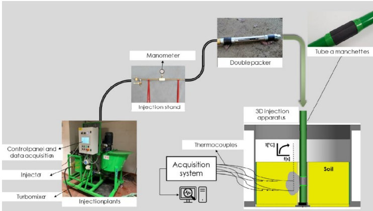
Fig. 14-2, ITS – Injection Tube System® allows to perform on real scale the permeation grouting treatment process in laboratory (Galli, 2023)
