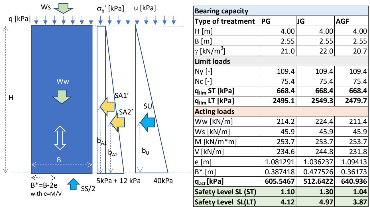
Fig. 6-6, Bearing capacity verification of the adopted case study (ST Short Term; LT long Term).
