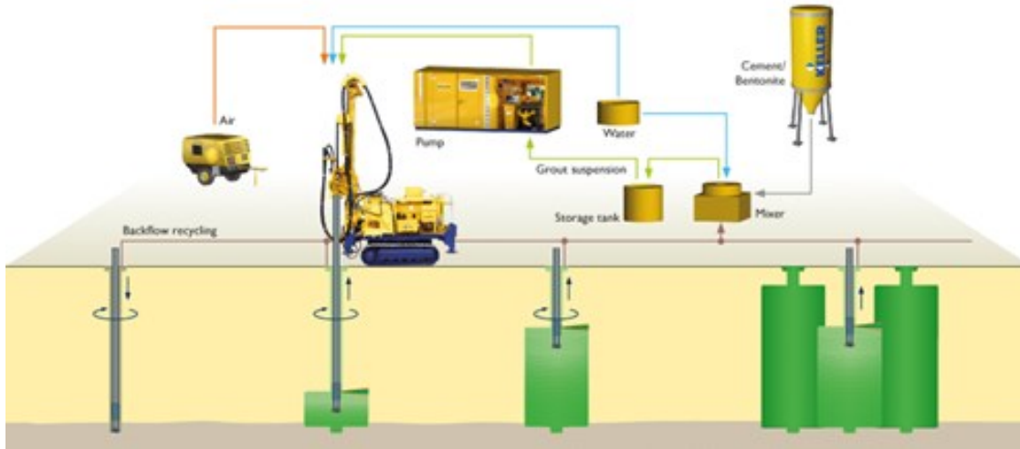
Fig. 7-4, A sitework equipment scheme for single and double fluid Jet Grouting technique (Keller). The air compressor is used only in the double fluid system
