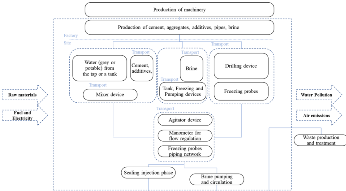
Fig. 18-19, Artificial ground freezing with brine technique: Process scheme for LCA Analysis.
