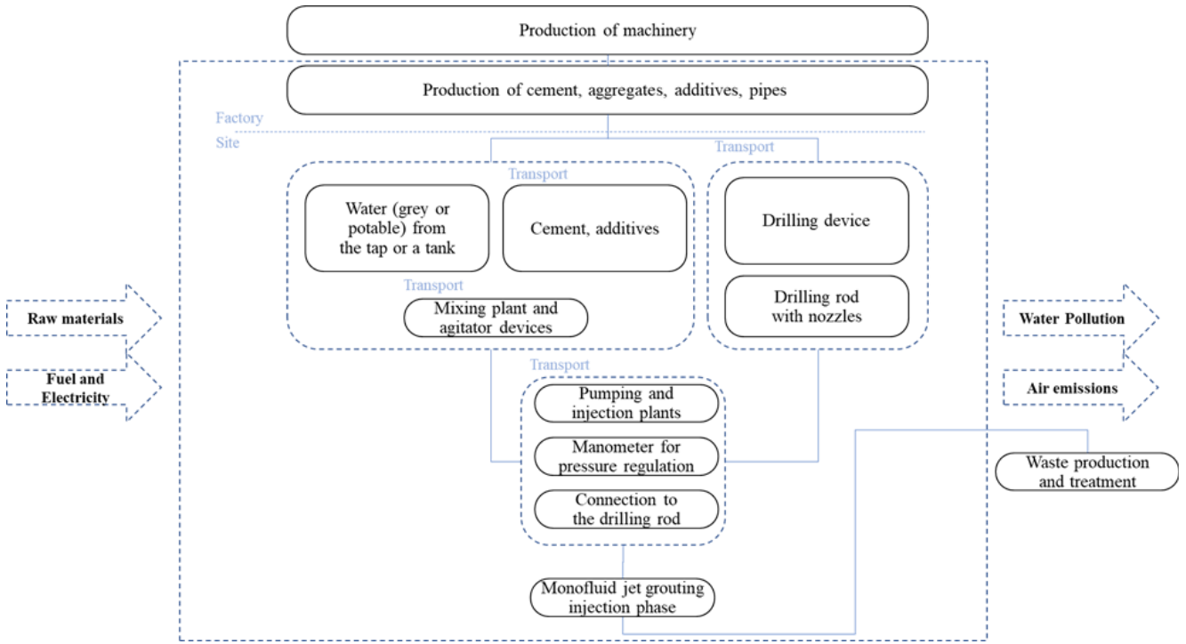
Fig. 18-7, Process scheme for LCA Analysis of the single fluid Jet Grouting technique.
