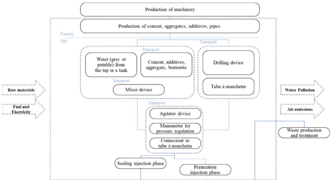
Fig. 9-4, Process scheme for LCA Analysis of the permeation grouting technique.
