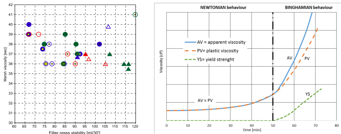
Fig. 14-1 Laboratory preliminary test on grouts rheological parameters – on the left Marsh viscosity vs. filter press stability of cement grouts; on the right viscosity vs. groutability time for silica grouts (Pettinaroli et al., 2019)
