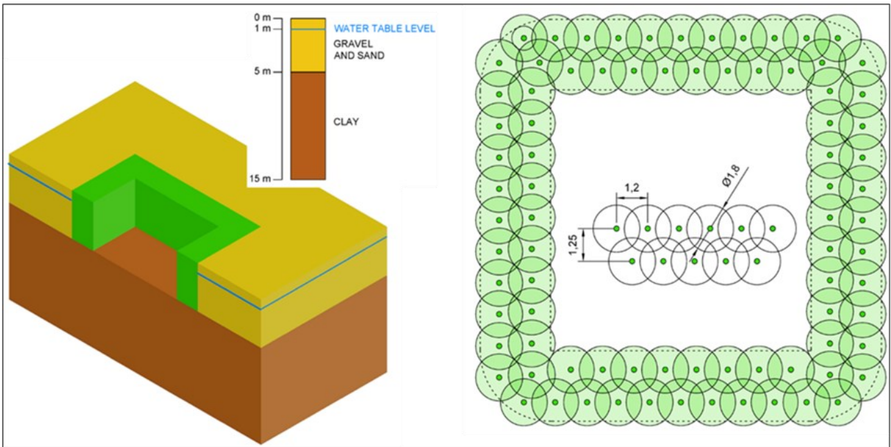
Fig. 9-3, Permeation grouting treatment: geometrical data.
