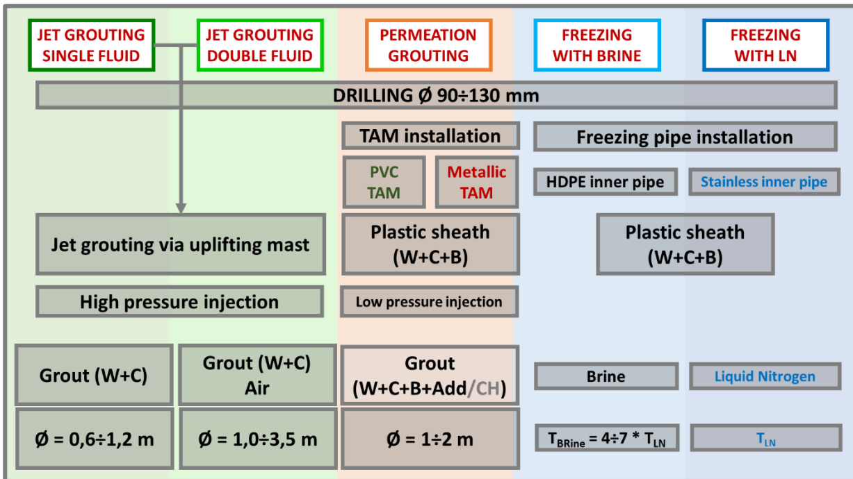
Fig. 7-1, The main characteristics of the ground improvement technologies considered for the pilot case analysis
