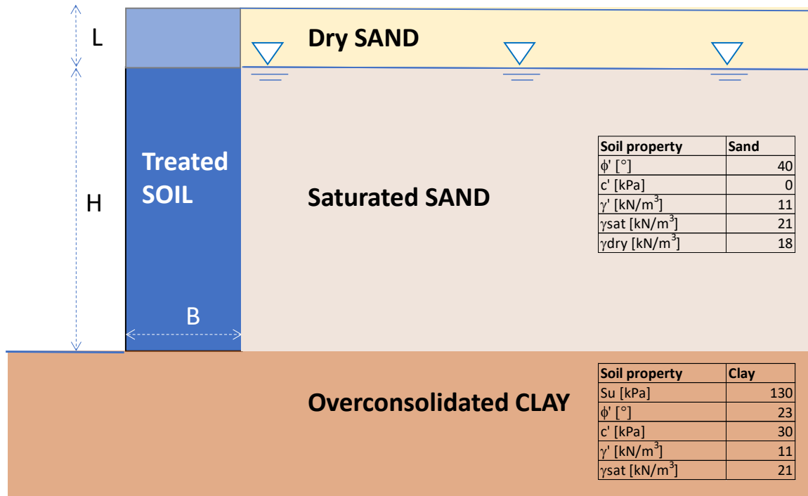
Fig. 6-3, Layout and geotechnical properties of the case study.
