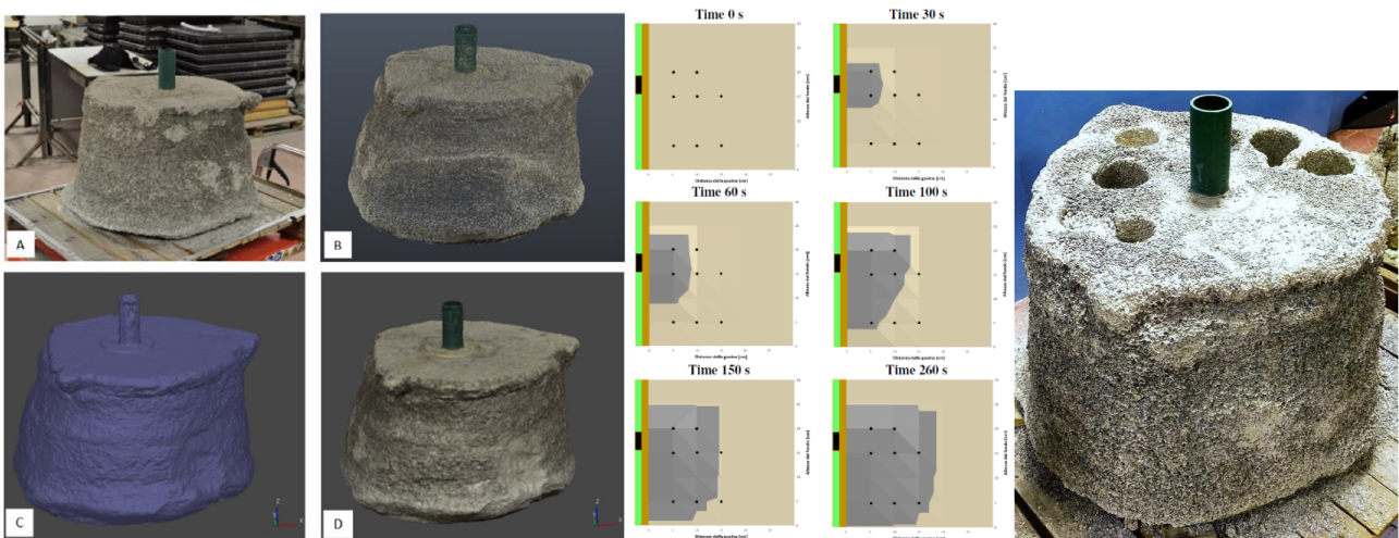
Fig. 14-3, ITS ® - left: photogrammetry and laser scansion for determining the treated soil volume – center: grout diffusion in the soil measured by thermometric sensors – treated soil after specimens sampling (Galli, 2023)
