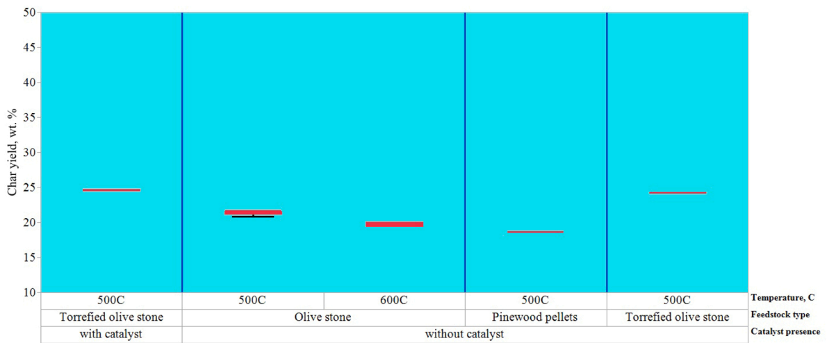
(b): Char distribution
