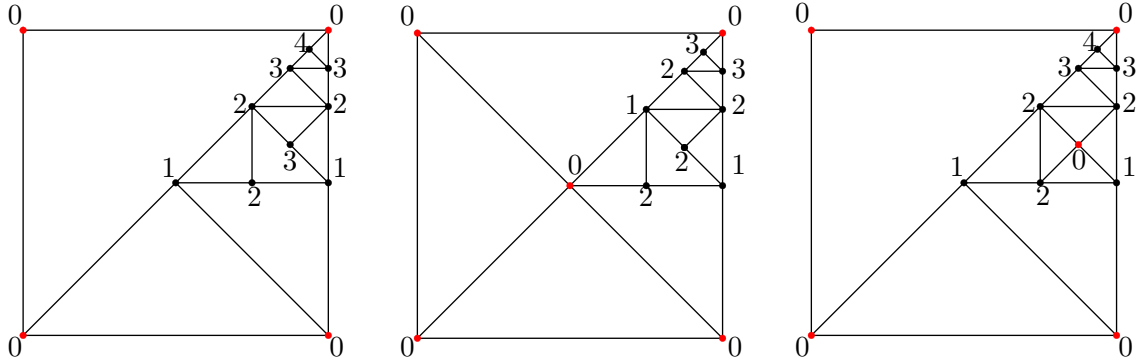
Figure 1: Three examples of distributions of proper nodes (red) and hanging nodes (black), with associated global indices \lambda . The bisection added in the middle picture converts the centered node into proper, and induces nonlocal changes of global indices on chains associated with it. If \Lambda = 3 , then the leftmost mesh is not admissible and this procedure is instrumental to restore admissibility. The right picture illustrates the creation of a proper node without nonlocal effects on global indices.
