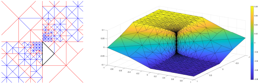
Figure 12: Test 2. Left: final grid \mathcal{T}_{\text{VEM}} , zoom to (-10^{-10}, 10^{-10})^2 (mesh elements having more than three vertices are drawn in red, and the mesh element drawn in black is a nonagon). Right: graph of the discrete solution.
