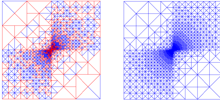
Figure 10: Test 2. Left: final grid \mathcal{T}_{\text{VEM}} obtained with VEM. Right: final grid \mathcal{T}_{\text{FEM}} obtained with FEM. Mesh elements having more than three vertices are drawn in red.
