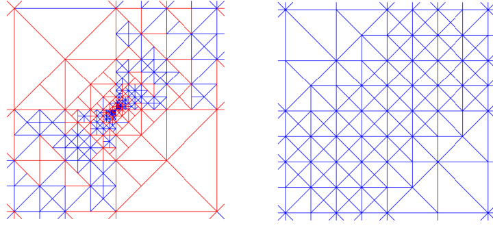
Figure 11: Test 2. Left: final grid \mathcal{T}_{\text{VEM}} . Right: final grid \mathcal{T}_{\text{FEM}} . Zoom to (-10^{-9}, 10^{-9})^2 . Mesh elements having more than three vertices are drawn in red.
