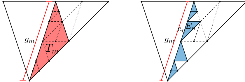
Figure 5: The edge g_m of the ancestor T_m of E (left). The partition of g_m into edges e_n of elements E_n \in \mathcal{T} (right)
