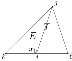
Figure 3: Sample of element E \in \mathcal{T} , where T = A(E) is the parent of E , i, j, k are the global indices of the vertices of E ( i being the global index of \mathbf{x}_0 ), and \ell is global index of the remaining vertex of T .
