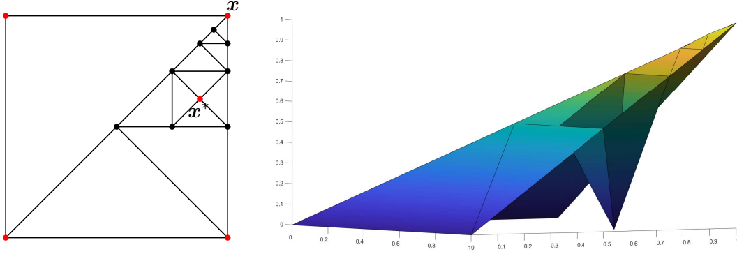
Figure 2: Left: detail of a mesh \mathcal{T} , in which red nodes \mathbf{x} and \mathbf{x}^* are proper nodes. Right: basis function \psi_{\mathbf{x}} \in \mathbb{V}_{\mathcal{T}}^0 ; notice that \psi_{\mathbf{x}}(\mathbf{x}^*) = 0 and the basis function \psi_{\mathbf{x}^*} \in \mathbb{V}_{\mathcal{T}}^0 is the usual hat function supported in the square centered at \mathbf{x}^* (not depicted).
