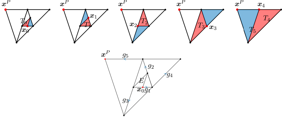
Figure 4: The chain of ancestors of E = T_0 leading to T_5 having a proper node as a vertex (above). The path g_1 \rightarrow g_2 \rightarrow \dots \rightarrow g_5 connecting \mathbf{x}_0 \in E to the proper node \mathbf{x}^P \in T_5 (below)
