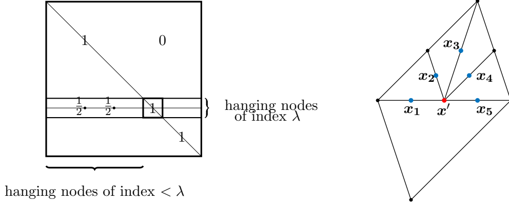
Figure 6: Left: structure of one factor \mathbf{W}_\lambda in the factorization (7.11). Right: given an hanging node \mathbf{x}' with \lambda(\mathbf{x}') < \lambda , at most 5 hanging nodes \mathbf{x}_i for i = 1, \dots, 5 of index \lambda may be such that \mathbf{x}' \in B(\mathbf{x}_i) .
