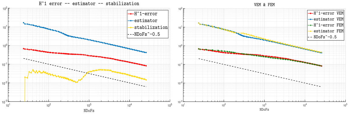
Figure 9: Test 2. Left: H^1 -error, estimator \eta_{\mathcal{T}}(u_{\mathcal{T}}, \mathcal{D}) , stabilization term S_{\mathcal{T}}(u_{\mathcal{T}}, u_{\mathcal{T}})^{1/2} . Right: H^1 -error and estimator \eta_{\mathcal{T}}(u_{\mathcal{T}}, \mathcal{D}) obtained with VEM and FEM. In both figures the optimal decay is indicated by the dashed line with slope -0.5 .
