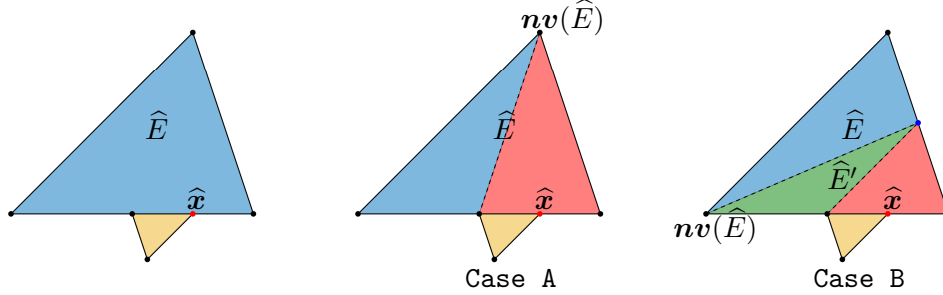
Figure 7: Left: mesh element \hat{E} having \hat{x} as hanging node, with \hat{x} such that \lambda(\hat{x}) = \Lambda_{\mathcal{T}} > \Lambda . Middle: case A the node \hat{x} belongs to the opposite edge to the newest-vertex of \hat{E} , therefore one bisection is needed. Right: case B the node \hat{x} belongs to the same edge of the newest-vertex of \hat{E} , therefore two bisections are needed.
