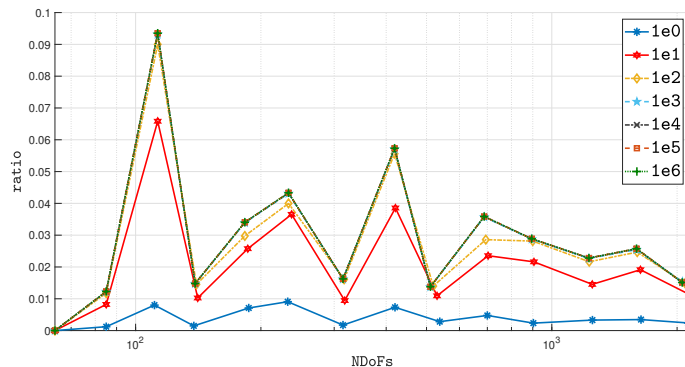
Figure 8: Test 1. Sharpness of bound (4.10): ratio between the term \gamma^2 S_{\mathcal{T}}(u_{\mathcal{T}}, u_{\mathcal{T}}) and the term \eta_{\mathcal{T}}^2(u_{\mathcal{T}}, \mathcal{D}) obtained with the adaptive algorithm (5.3).
