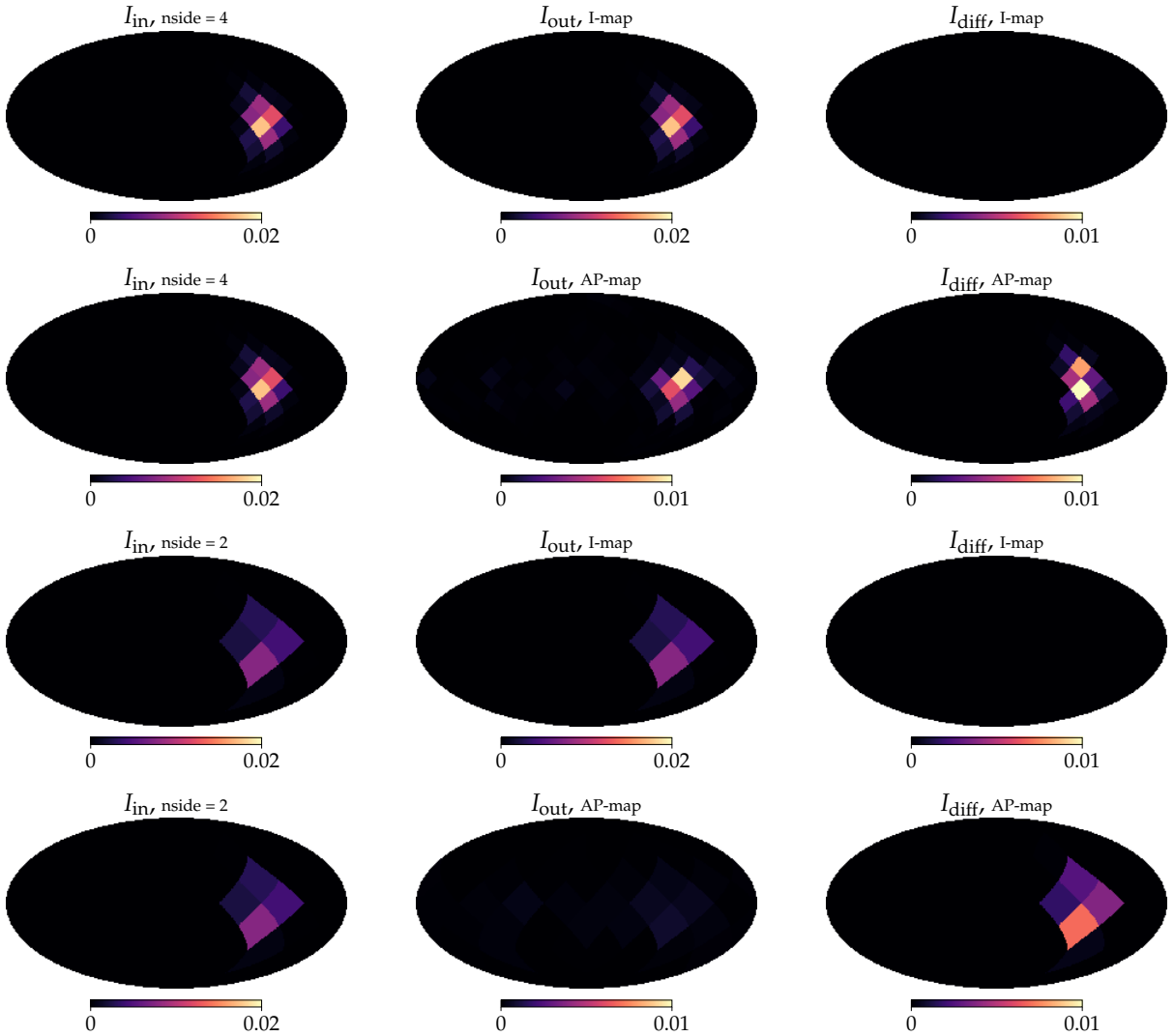
FIG. 3. A comparison between the recoveries of the same injected map I_{\text{in}} with the intensity I (first and third rows) and amplitude-phase AP (second and fourth rows) mapping algorithms, with the two different values of N_{\text{side}}^{\text{out}} as shown in Fig. 2. On the right, the difference maps I_{\text{in}} - I_{\text{out}} are shown to quantitatively comparative the performance of the algorithms. Note that the input map has been ud_graded to allow for this comparison; the actual input map is at N_{\text{side}} = 16 as shown in Fig. 1.
