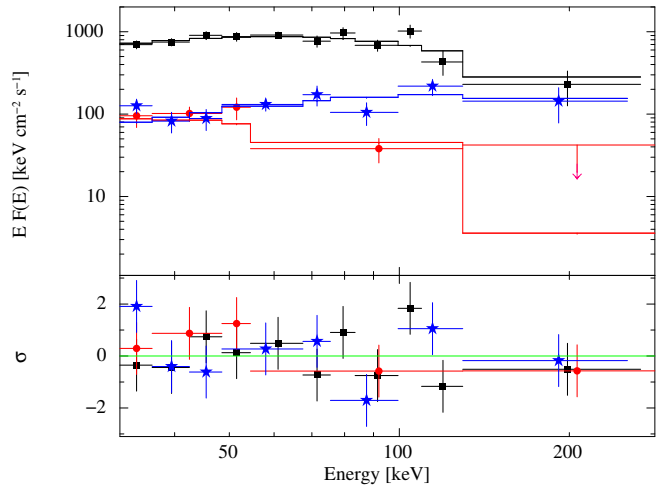
Figure 2. Unfolded energy spectra of burst-G fitted with a cut-off power law model (top panel). The three spectra refer to the main pulse (black squares), and to the intervals before (red circles) and after (blue stars) the main pulse. The spectra have been rebinned for plotting purposes. The lower panel shows the residuals in units of \sigma .
