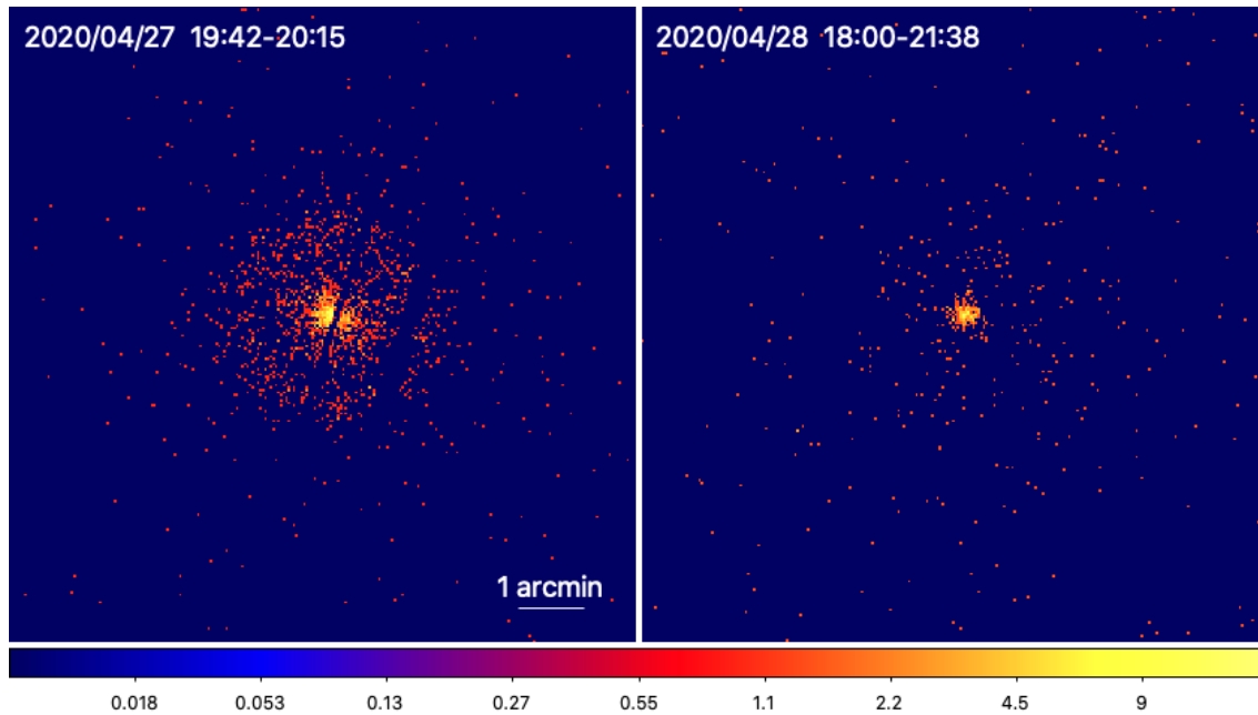
Figure 5. X-ray images (0.2-10 keV) of SGR 1935+2154 obtained with Swift/XRT on 2020 April 27 (ID 00968211001, left panel) and 28 (ID 00033349045, right panel). The first observation clearly shows a ring of scattered emission that extends for more than 1' from the source. The ring was no more visible the following day, owing to its fading X-ray flux and increasing angular radius.
