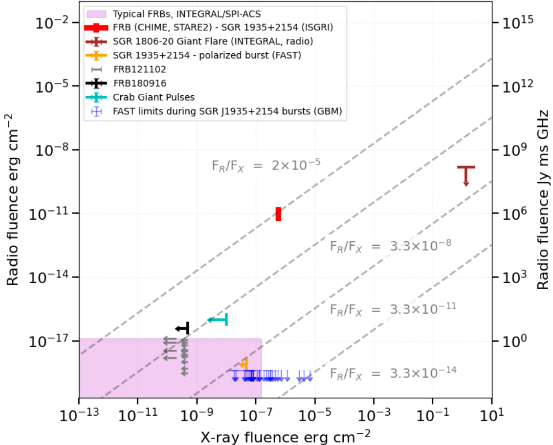
Figure 8. Radio versus X-ray (starting from 0.5 keV) fluences for FRBs and magnetar bursts. The range of FRB fluences corresponds to a variety of detections reported in the past years (references in Fig. 7 and Karuppusamy et al. 2010). The purple region indicates a robust upper limit on the hard X-ray fluence of FRBs as derived with a high-duty-cycle detector, such as the INTEGRAL SPI/ACS (Savchenko et al. 2017).
