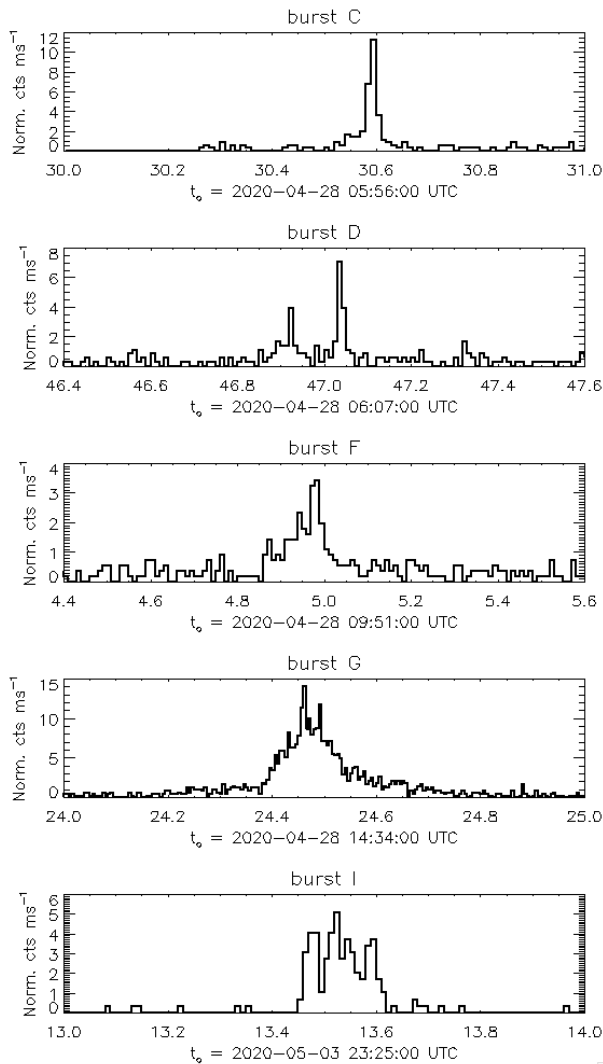
Figure 3. Light curves in the 20-200 keV range for the bursts of Table 2 with more than 100 counts. Time bins are of 10 ms, except for burst-G that is binned at 5 ms. The count rates have been normalized to the values that would have been obtained with the source on-axis.
