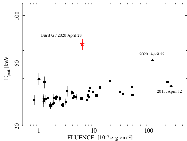
Figure 6. Peak energy versus fluence for Burst-G (red star) and other bursts from SGR 1935+2154 (squares from Lin et al. (2020a), triangles from Kozlova et al. (2016) and Ridnaia et al. (2020b)).
