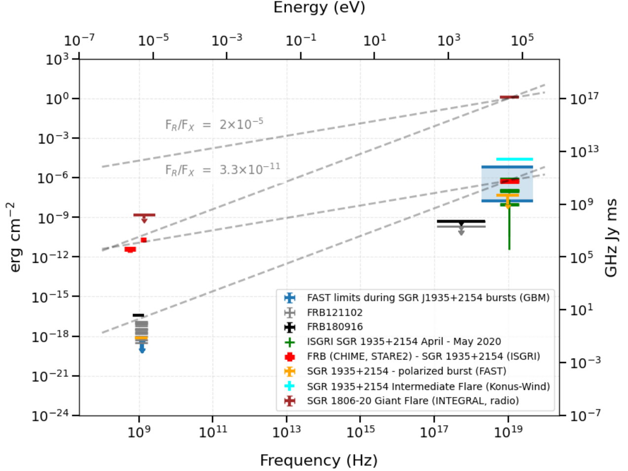
Figure 7. Comparison of the spectral energy distribution of burst-G from SGR 1935+2154 (red) with the upper limits for other magnetars and FRBs obtained from simultaneous radio and X-ray observations (Hurley et al. 2005; Tendulkar et al. 2016; Kozlova et al. 2016; Scholz et al. 2017; Lin et al. 2020b; The CHIME/FRB Collaboration et al. 2020a; Bochenek et al. 2020; Scholz et al. 2020; Pilia et al. 2020)
