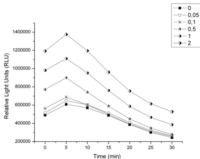
Fig. 3. Light emission by E. coli XL-1/pSak-lux from anaerobically grown cells induced with different concentrations of arabinose (% in the right corner box) as a function of time after aerobic incubation. The values are the means of two independent experiments conducted in triplicates. The variation between the replicates was less than 10%.
