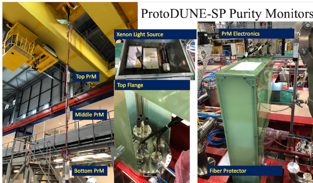
Figure 8.17. The ProtoDUNE-SP purity monitoring system.
