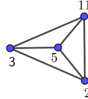
Figura 3. \Delta^*(M_{11})
