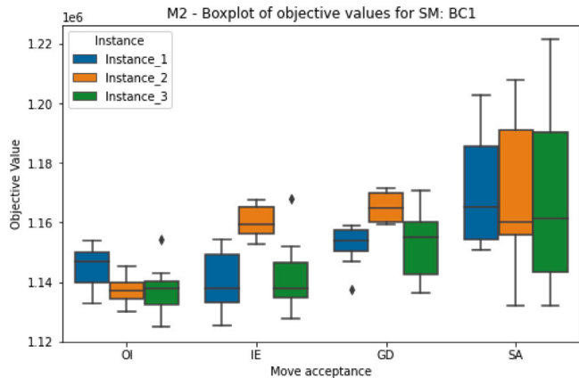
Fig. 13. Model 2 boxplot for selection method Best Choice 1 for Instance 1, 2 and 3.
