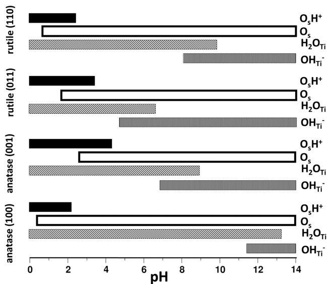
Figure 4. pH windows at which the \text{H}^+ , \text{O}_s , \text{H}_2\text{O} , and \text{OH}^- species are present on the surface. A threshold molar fraction of 10% has been adopted.
