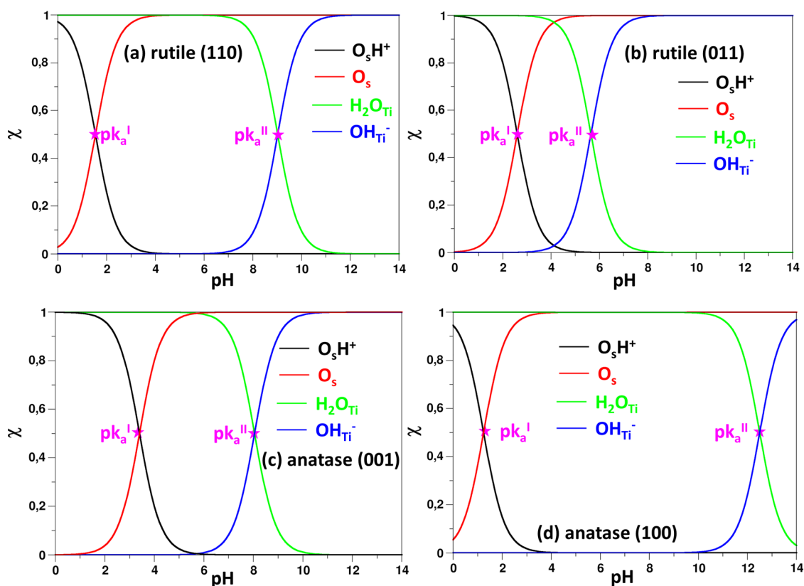
Figure 3. Speciation of adsorbed water ( \text{H}_2\text{O} ), free surface oxygen sites ( \text{O}_s ), and \text{H}^+ and \text{OH}^- species as a function of pH on the surface of (a) rutile (110), (b) rutile (011), (c) anatase (001), and (d) anatase (100).
