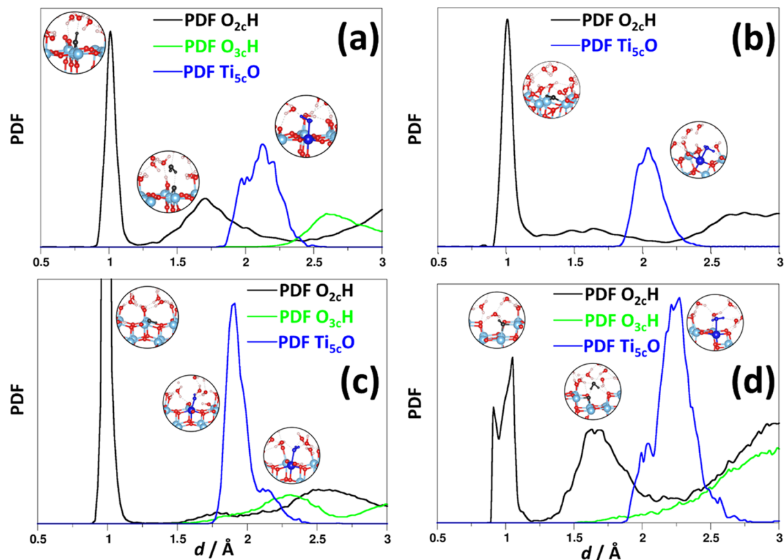
Figure 2. Calculated pair distribution function (PDF) between O_{2c} and H atoms (black solid line), O_{3c} and H atoms (green solid line), and surface Ti and O atoms of water (blue solid line) for TiO_2 /water interfaces. (a–d) Rutile (110), rutile (011), anatase (001), and anatase (100), respectively.
