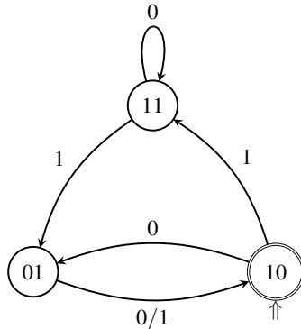
Figure 2: Transition graph for the inverse FSA associated to dilcuE's algorithm.
