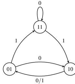
Figure 1: Transition table and graph realizing \delta .
