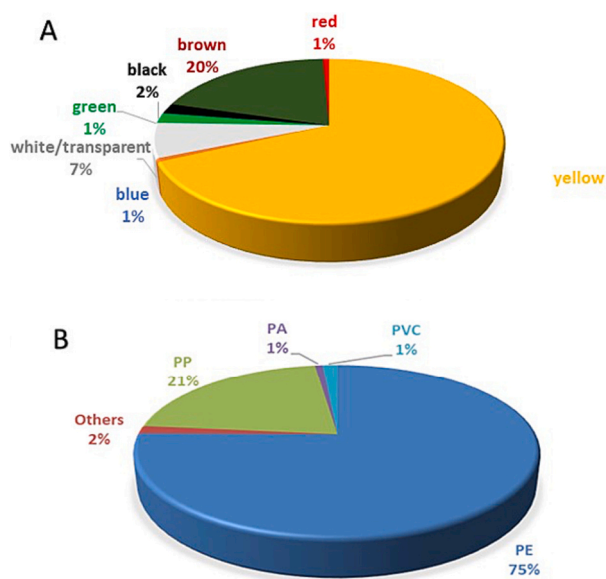
Fig. 3. Colors (A) and polymers (B) of the plastic particles extracted from Mediterranean plastitar samples. PA = Polyamide; PVC = polyvinylchloride; PE = polyethylene; PP = polypropylene.
