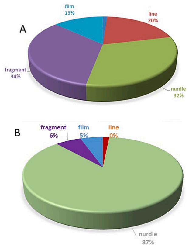
Fig. 4. Particle shape distribution observed in all plastic items extracted from Mediterranean plastitar samples (A) and only in the microplastic particles (B).
