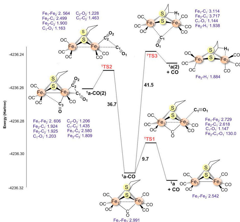
Figure 4. Total density functional theory (DFT) energy diagram and optimized main geometry parameters of ^1a\text{-CO} and cis\text{ syn, trans syn} and \mu\text{-CO} CO dissociation transition states and products. The energy in Hartree and free-energy barriers in kcal·mol -1 . Distances are in Å and angles in degrees.
