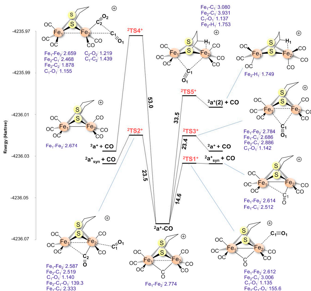
Figure 5. Total DFT energy diagram and optimized main geometry parameters of {}^2a^+-CO and cis syn , trans syn and \mu -CO CO dissociation transition states and products. The energy in Hartree and free-energy barriers in kcal·mol -1 . Distances are in Å and angles in degrees.
