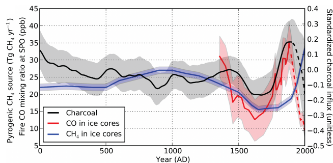
Figure 5. Variability of biomass burning rates over the last centuries based on a worldwide compilation of charcoal records (Marlon et al., 2008), CO mixing ratios from fires using CO concentration measurements at the South Pole (SPO), its isotopic signature, and a mass balance model (Wang et al., 2010), as well as a similar approach but based on \text{CH}_4 (Ferretti et al., 2005). The CO ice core data ended in 1897 but were extended (dashed line) by Wang et al. (2010) to the present day using firn samples (1968 and 1986) as well as modeling (year 2000). Shaded areas indicate reported uncertainty. Note that the datasets have different footprints and that absolute values cannot be compared directly. Reproduced with permission from van der Werf et al. (2013) under CCC3.0.
