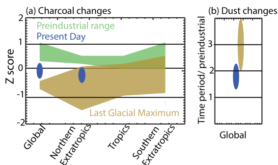
Figure 6. Relative size of paleoclimate and historical changes in aerosols. (a) Based on z scores from charcoal records, the variability across preindustrial time periods (green), the present day (blue), and the Last Glacial Maximum is shown globally as well as for the northern extratropics, tropics, and southern extratropics based on data from Marlon et al. (2008, 2016). Charcoal reconstructions use z scores, which are normalized by the mean value at a site, divided by the variability, and thus a -2z score for LGM suggests significantly lower charcoal amounts. (b) Global dust change ratio of deposition between the present day and preindustrial (blue oval; Mahowald et al., 2010; Kok et al., 2023) and for the Last Glacial Maximum relative to the preindustrial (gold oval) (Mahowald et al., 1999; Albani et al., 2014, 2018; Lambert et al., 2015).
