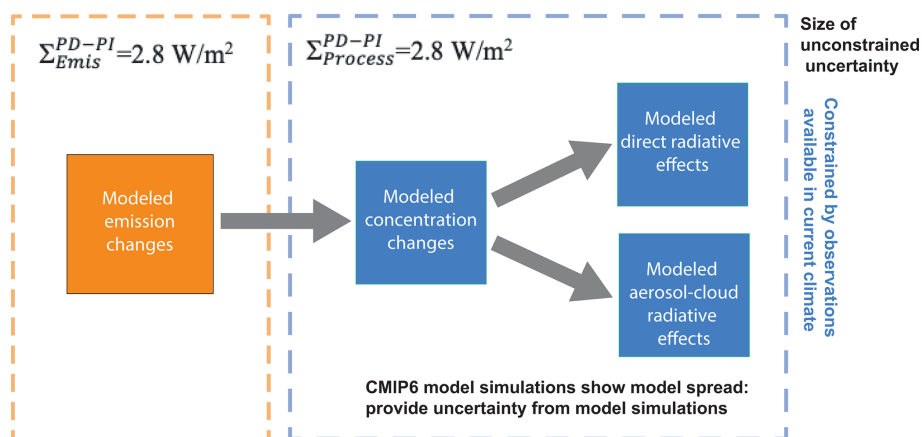
Figure 3. Schematic of the sources of uncertainties in aerosol radiative effects from emission models to modeled concentration changes to modeled direct and aerosol–cloud radiative effects. The CMIP6 unconstrained uncertainties using a single emission scenario have a 90 % confidence interval range of 2.8 \text{ W m}^{-2} (Bellouin et al., 2020; Sherwood et al., 2020). For the uncertainty summed over different aerosol species ( \Sigma ) using different emission scenarios for the past climate, the 90 % confidence interval ranges from wildfires of 2.8 \text{ W m}^{-2} (Hamilton et al., 2018; Wan et al., 2021) is added in quadrature to uncertainties from dust of 0.4 \text{ W m}^{-2} (Kok et al., 2023) and an estimate of industrial emission uncertainties (assuming 10 % error) of 0.2 \text{ W m}^{-2} , obtaining a 2.8 \text{ W m}^{-2} uncertainty in emissions.
