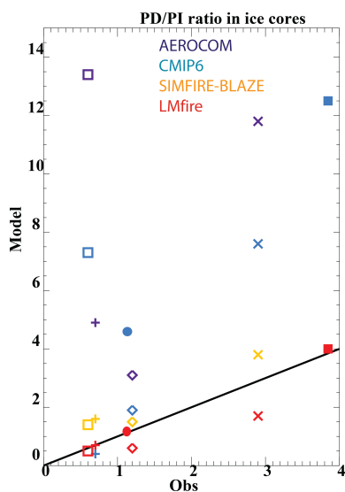
Figure 2. Observed and modeled present-day to preindustrial ratios (PD/PI) for black carbon in ice cores using different open fire emissions. Ice core sites are from Greenland (open square and plus signs), Wyoming (diamond), and France (x symbols) for four different model simulations: AEROCOM (purple), CMIP6 (blue), SIMFIRE-BLAZE (yellow), and LMfire (red) are taken from Hamilton et al. (2018). Ice core sites from Bolivia (solid circle) and Antarctica (solid square) using CMIP6 (blue) and LMfire (red) are taken from Liu et al. (2021). The solid black line shows the 1 : 1 line.
