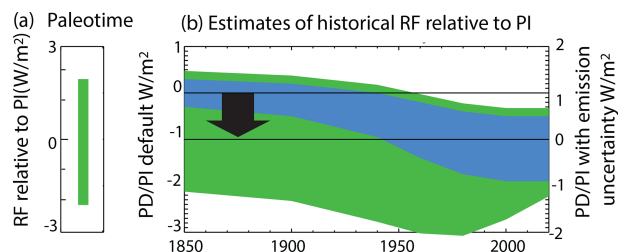
Figure 4. Estimates of the unconstrained aerosol radiative forcing and its uncertainties for (a) different paleoclimate time periods relative to the preindustrial (PI; 1850) and (b) present day (PD) relative to 1850 based on CMIP6 model spread (schematic based on Smith et al., 2021, in blue) and including the emission uncertainties (90 % confidence intervals) from wildfires, dust, and anthropogenic aerosols as described in Fig. 3 (green) using the time series for wildfires from Marlon et al. (2008). The left vertical axis represents the present-day minus preindustrial radiative forcing (blue area) following Smith et al. (2021) and Sherwood et al. (2020), and the right axis adds in the emission uncertainties for the preindustrial (from Fig. 3; Hamilton et al., 2018), shifting the preindustrial baseline of aerosol radiative effects (black arrow; green area). Notice that the size of the black arrow and shift in the preindustrial state is not known, and this is a schematic to illustrate how the uncertainties in emissions in the preindustrial impact understanding of the radiative forcing.
